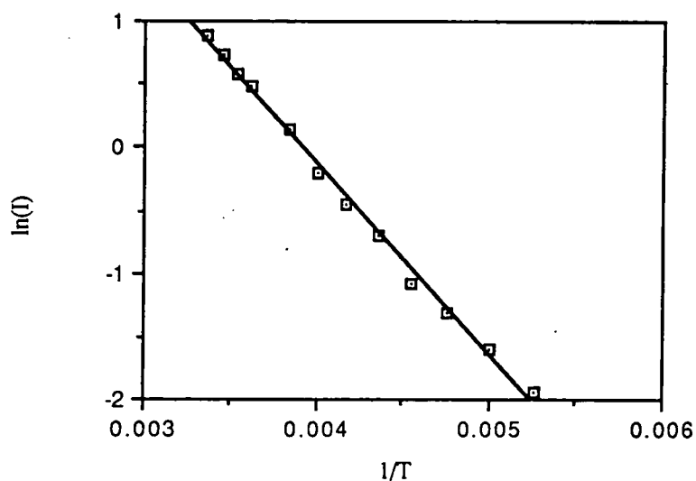
Figure (5.25) A plot of \log(I) vs 1/T for the low temperature data
