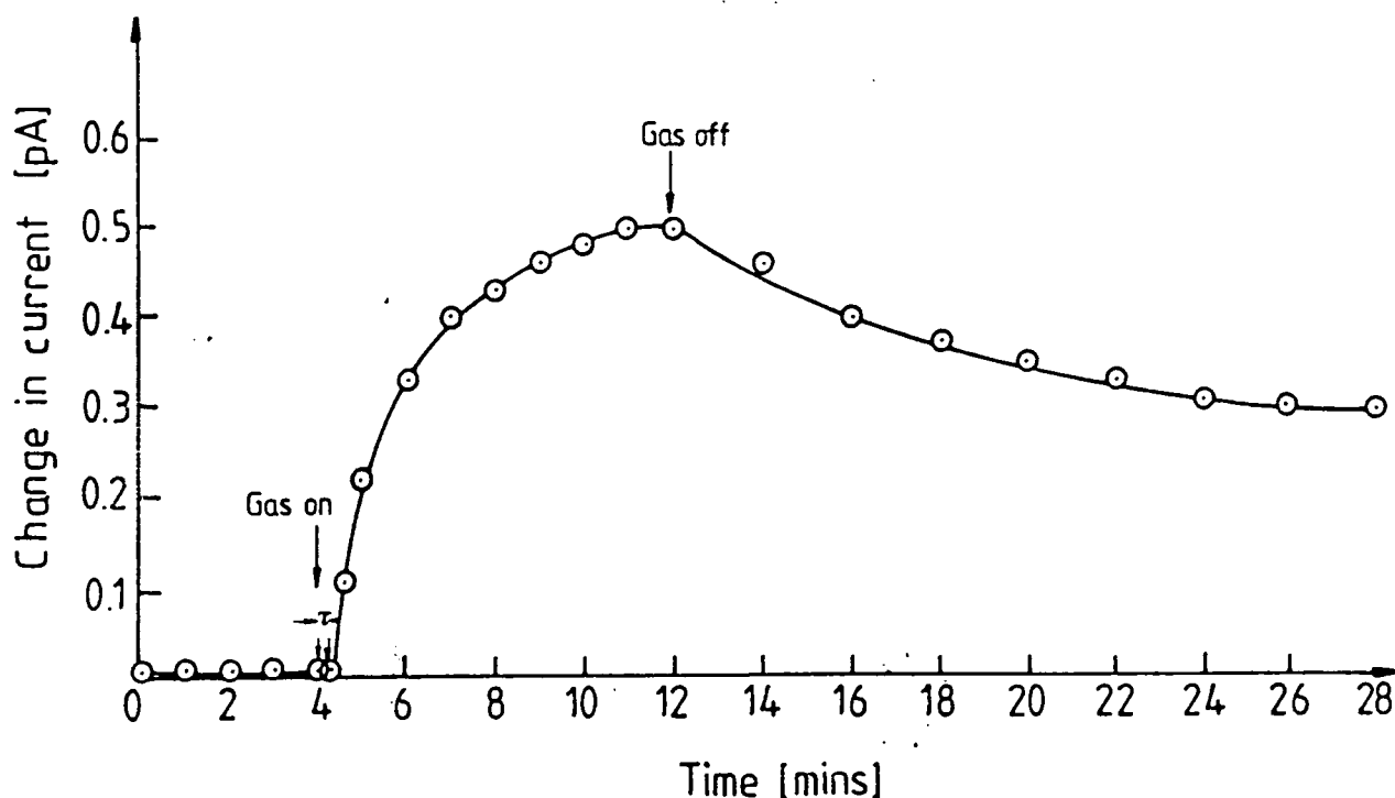
Figure 5.17a: The effect of 10ppm \text{SO}_2 on an evaporated polyaniline chemiresistor (2V supply and film thickness 210nm).
