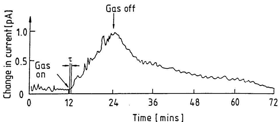
Figure 7.8a: The effect of 9ppm NO x on 7 LB layers of a LuPc 2 chemiresistor (3V supply).
