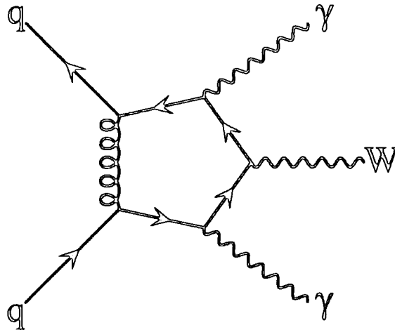
Fig.3.6.4 One of the pentagon Feynman diagrams that contributes to the NLO calculation of p\bar{p} \rightarrow W\gamma\gamma .
