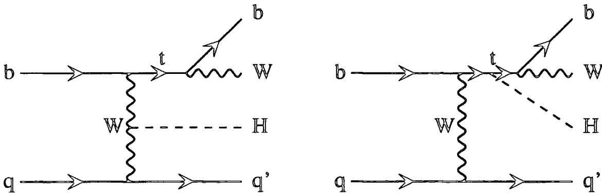
Fig.3.8.1 The Feynman diagrams for qb \rightarrow tHq' \rightarrow bWHq' .
