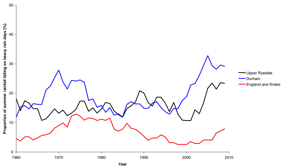
Figure 4.9: The proportion of summer rainfall falling on heavy rain days at upper Ryedale, Durham and England and Wales, showing ten year running means from 1960-2009. Upper Ryedale rainfall series formed from data contained in the Met Office MIDAS database. England and Wales Precipitation Series downloaded from the Met Office Hadley Centre website. England and Wales Precipitation Series data: © Crown Copyright 2011, dataset reference: Alexander and Jones, 2001. Durham rainfall data provided by Professor Tim Burt.
