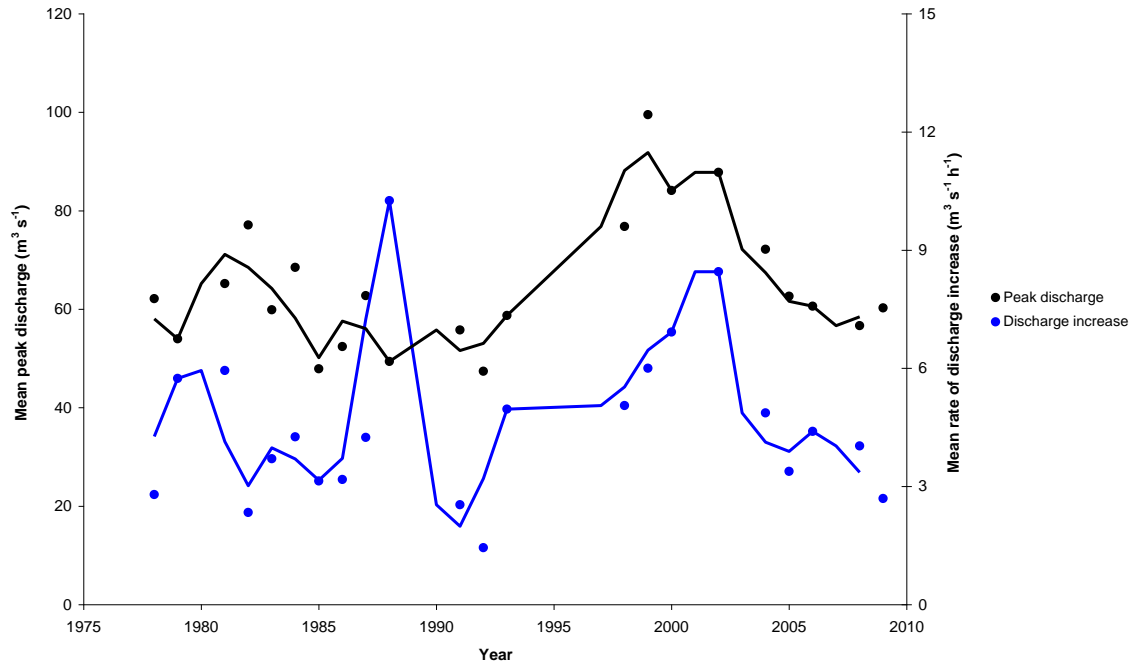
Figure 5.7: Comparison of the characteristics of high flows recorded at Broadway Foot, upper Ryedale, 1978-2009. High flows defined as the 50 largest flow events recorded in the Broadway Foot record ( 47.4 \text{ m}^3 \text{ s}^{-1} and above) with the 19th June 2005 flash flood not included in the data analysis. Figures used are annual means. Lines show two year running averages. Discharge data provided by the Environment Agency.
