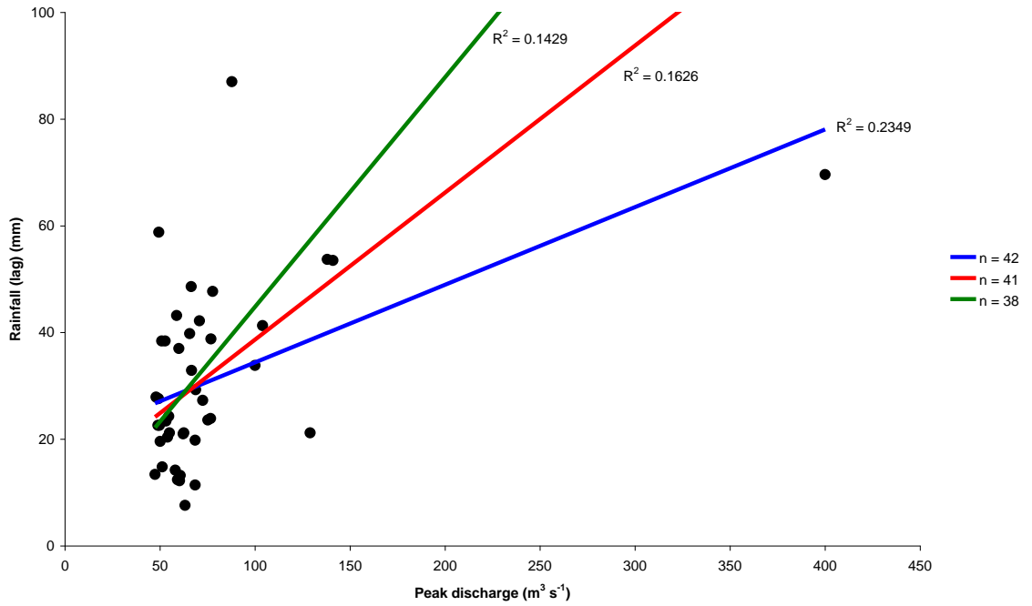
Figure 5.15: Relationships between peak discharge and rainfall for the largest flow events recorded at Broadway Foot, 1978-2009. Rainfall data formed from data contained in the Met Office MIDAS database, discharge data provided by the Environment Agency except 19th June 2005 peak discharge (estimate by Wass et al., 2008).
