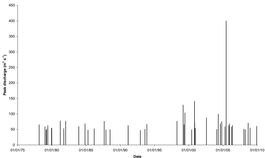
Figure 5.6: The 50 largest river discharge events recorded on the River Rye at Broadway Foot gauging station, 1978-2009. Discharge data provided by the Environment Agency, except 19th June 2005 peak discharge (estimate by Wass et al., 2008).
