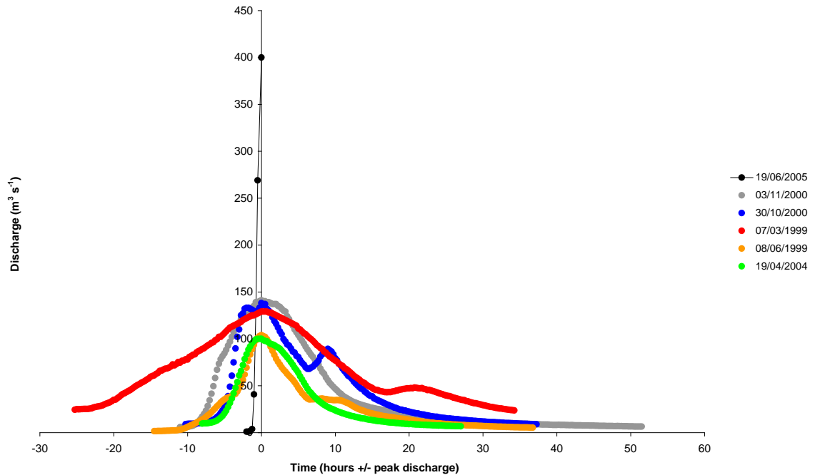
Figure 5.8: Comparison of the six largest discharge events recorded on the River Rye at Broadway Foot, 1978-2009. The flash flood event (19th June 2005) is shown with a black line for clarity. Discharge data provided by the Environment Agency, except 19th June 2005 peak discharge (estimate by Wass et al. , 2008).
