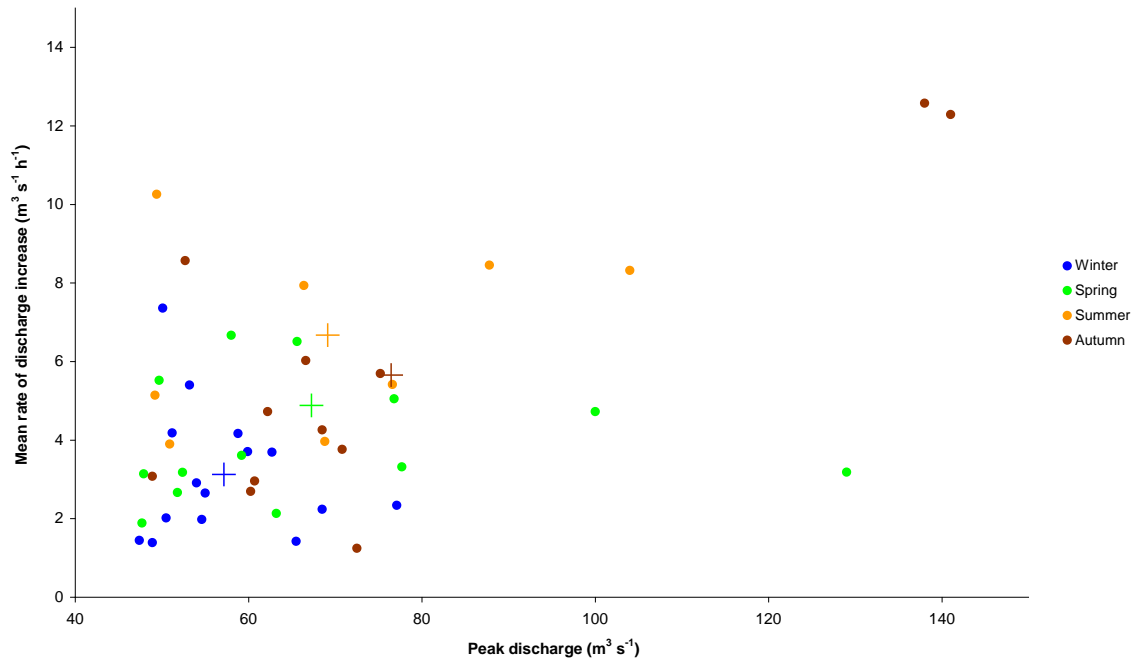
Figure 5.13: The peak discharges and mean rates of discharge increase for the 50 largest flow events recorded at Broadway Foot, upper Ryedale, 1978-2009. Events are categorised by the season in which they occurred. The mean centroids for each season are shown by cross marks (+) on the graph. The summer mean centroid does not take into account of the 2005 flash flood. Not all events are shown on the graph, including the 2005 flash flood. Discharge data provided by the Environment Agency.
