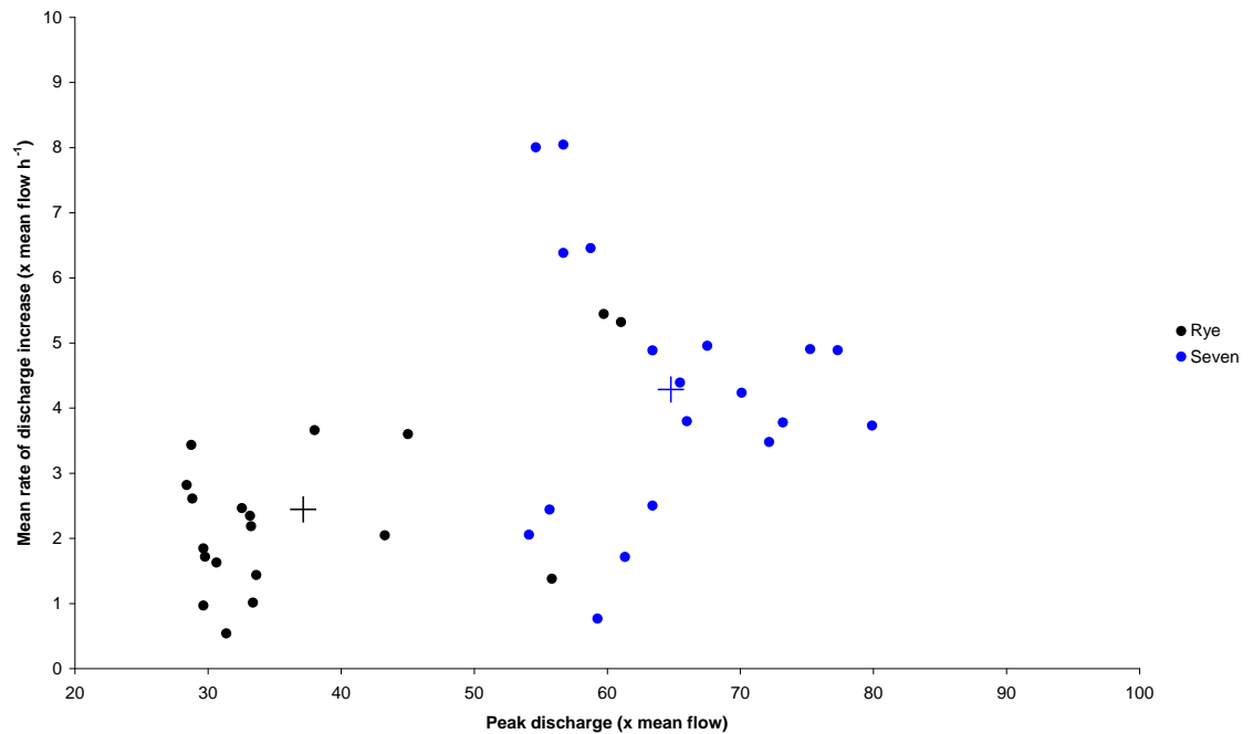
Figure 6.3: Comparison of the 20 largest discharge events recorded on the River Rye at Broadway Foot, and the River Seven at Normanby (shown on Figure 6.2). The events shown are those described in Table 6.1, minus the largest discharge event recorded at each station, with mean centroids shown as crosses. Not all events are shown. Discharge data provided by the Environment Agency.
