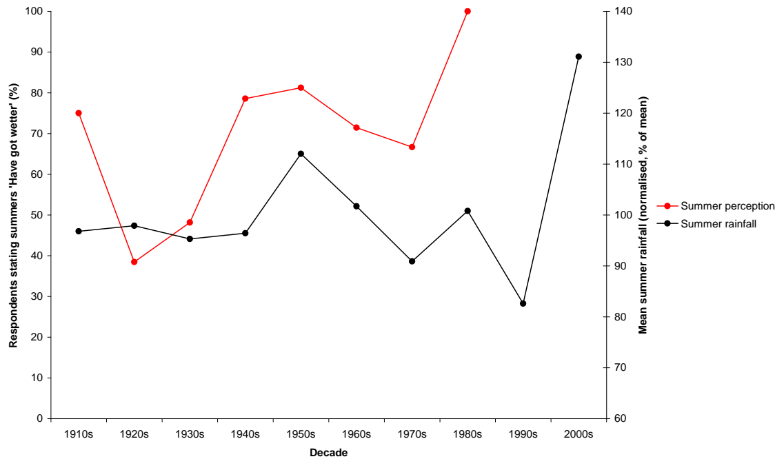
Figure 4.17: Comparison of the percentage of questionnaire respondents born in each decade who thought that summers 'have got wetter' over the time that they have lived in Ryedale, and the mean normalised summer rainfall totals for each decade/period. For perception of summer rainfall, n = 92 . The 1910s and 2000s are not complete decades. Summer rainfall data derived from the upper Ryedale rainfall series, which was formed from data contained in the Met Office MIDAS database.
