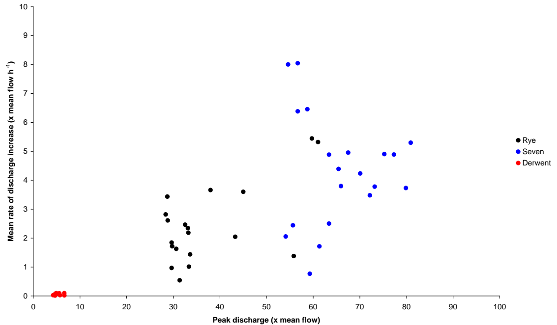
Figure 5.12: The characteristics of the 20 largest flow events recorded on the upland River Rye (at Broadway Foot) and River Seven (at Normanby) catchments between 1978 and 2009, and the ten largest flow events recorded on the River Derwent (at Malton) between 2003 and 2009. Not all events are shown, however all Malton events are shown. Discharge data provided by the Environment Agency.
