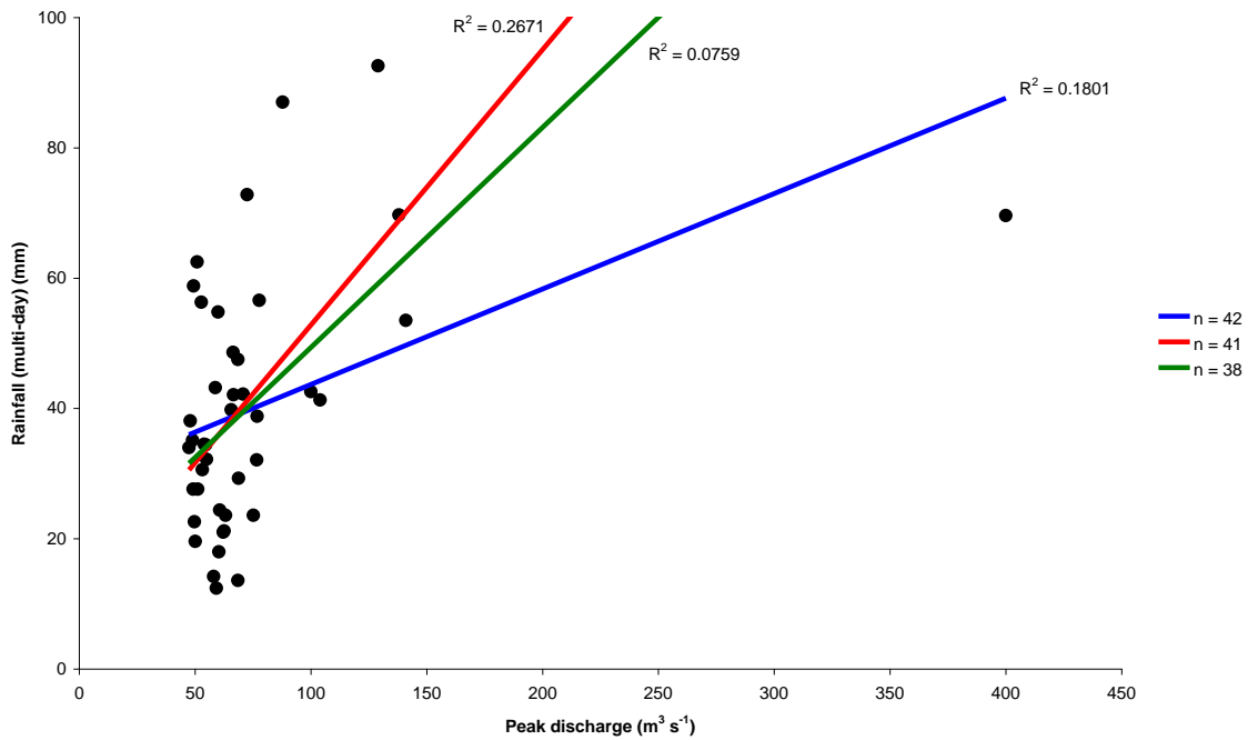
Figure 5.16: Relationships between peak discharge and multi-day rainfall for the largest flow events recorded at Broadway Foot, 1978-2009. Rainfall data formed from data contained in the Met Office MIDAS database, discharge data provided by the Environment Agency except 19th June 2005 peak discharge (estimate by Wass et al., 2008).
