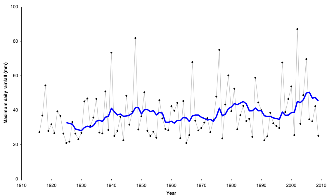
Figure 4.3: The maximum daily rainfall recorded annually at upper Ryedale, 1916-2009, showing ten year running mean. Rainfall series formed from data contained in the Met Office MIDAS database.
