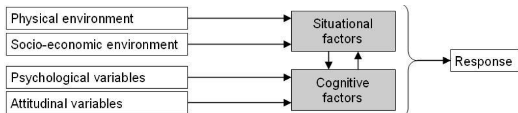
Figure 2.3: Factors influencing the perception of hazards. Diagram reproduced (and slightly adapted) from Tobin and Montz (1997), page 149.
