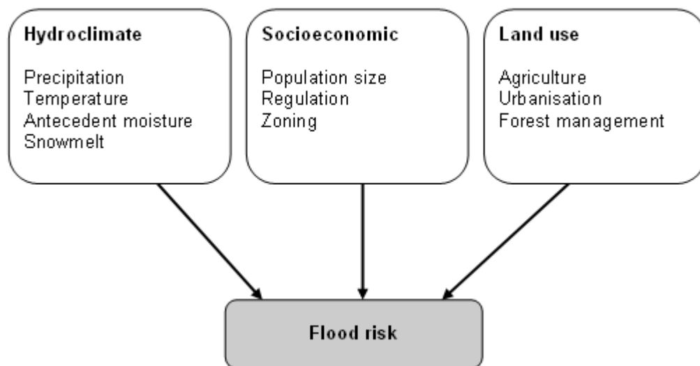
Figure 2.1: Factors influencing flood risks. Diagram redrawn from Chang and Franzyk, 2008, page 1550.
