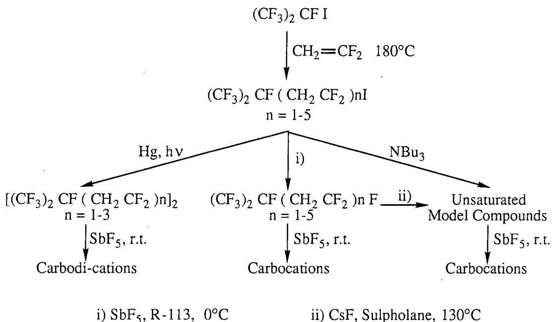
Scheme 1. Synthesis of model compounds as precursors for the carbocations
