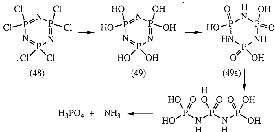
Scheme 5. Hydrolysis of hexachlorocyclotriphosphazene.
