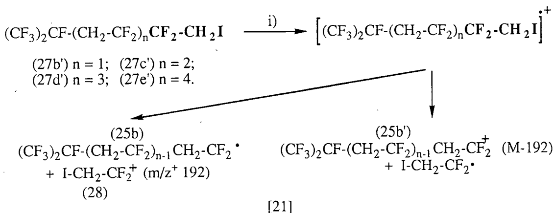
Scheme 3. Typical GC/MS fragmentation pattern of regio-isomers (27).
