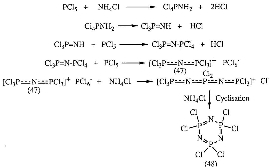
Scheme 4. Suggested mechanism for the formation of hexachlorocyclotriphosphazene.
