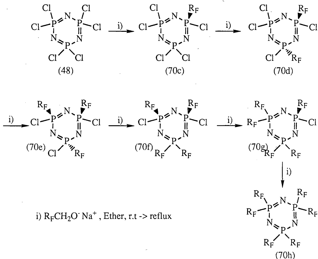
Scheme 9. Suggested mechanism for replacement of chlorine by perfluoroalkylpolyether-alkoxy groups in (48).
