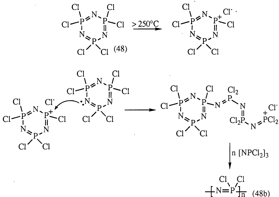
Scheme 7. Mechanism for ionic polymerisation of hexachlorocyclotriphosphazene.
