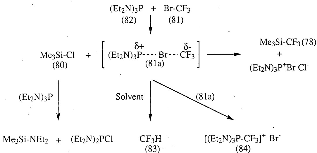
Scheme 11. Mechanism for the synthesis of \text{Me}_3\text{SiCF}_3
