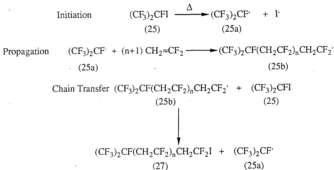
Scheme 2. Suggested mechanism for the telomerisation of vinylidene fluoride, using heptafluoroisopropyl iodide as a telogen.
