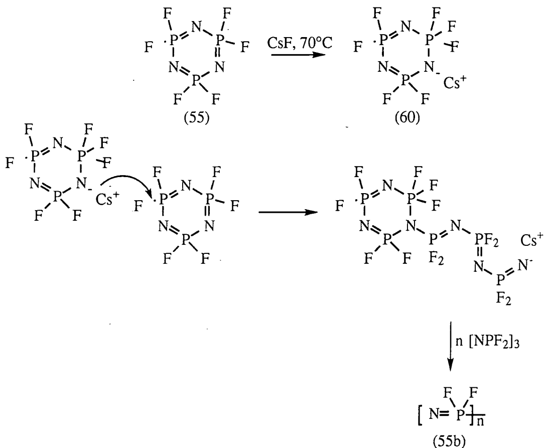
Scheme 8. Suggested mechanism for fluoride ion induced polymerisation of hexafluorocyclotriphosphazene
