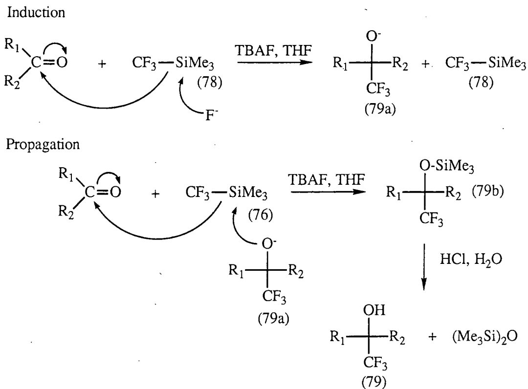
Scheme 10. \text{CF}_3\text{SiMe}_3 : a new trifluoromethylating agent.
