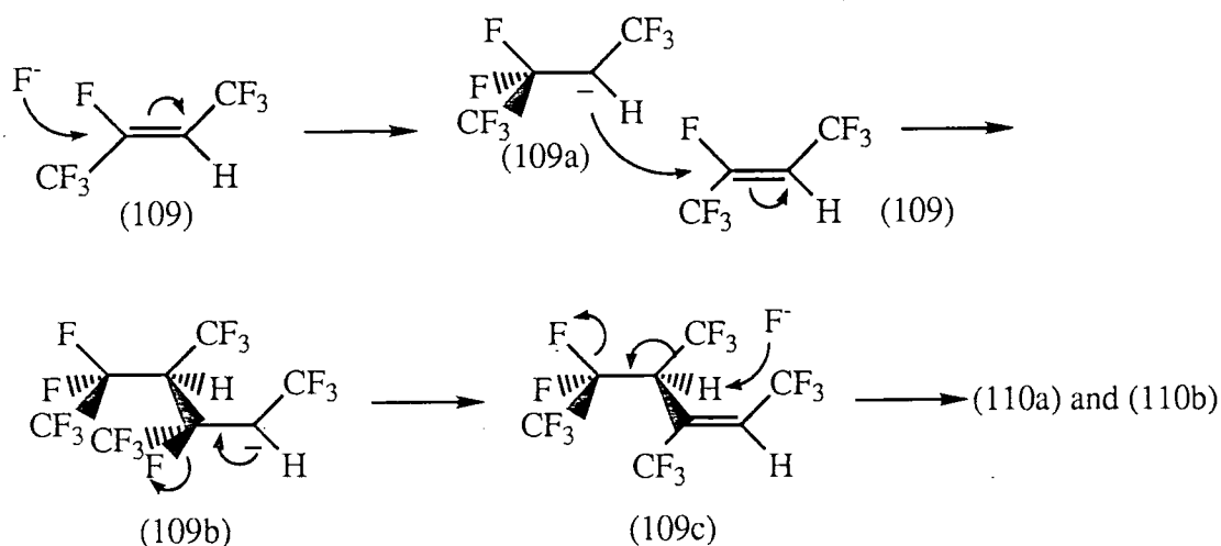
Scheme 13. Suggested mechanism for the formation of dimers (110).
