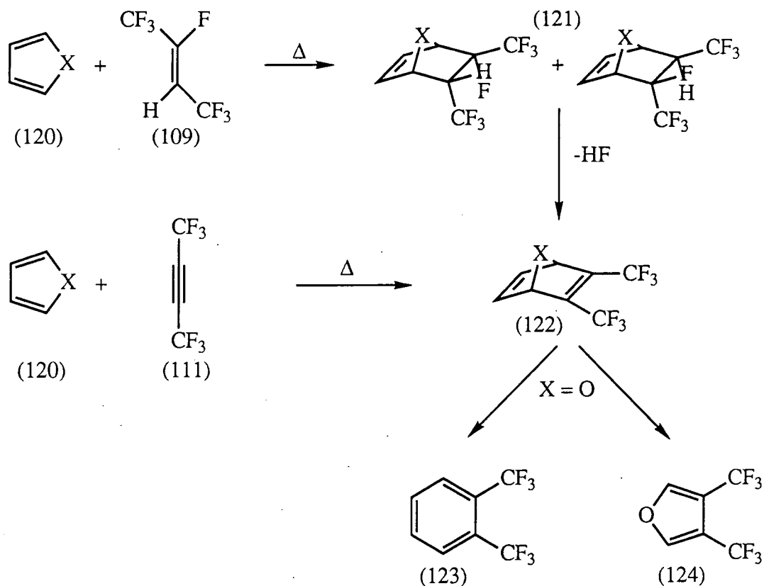
Scheme 15. 2-Hydroheptafluorobut-2-ene as a synthon for hexafluorobut-2-yne.
