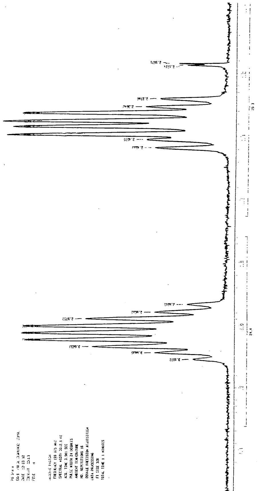
Figure 7. Expansion of the ^1\text{H} n.m.r spectrum of (131).
