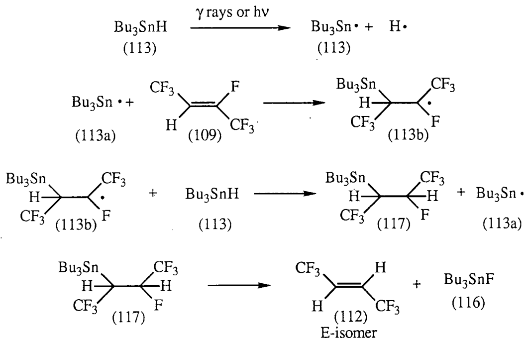
Scheme 14. Suggested mechanism for the synthesis of 2,3-dihydrohexafluorobut-2-ene.
