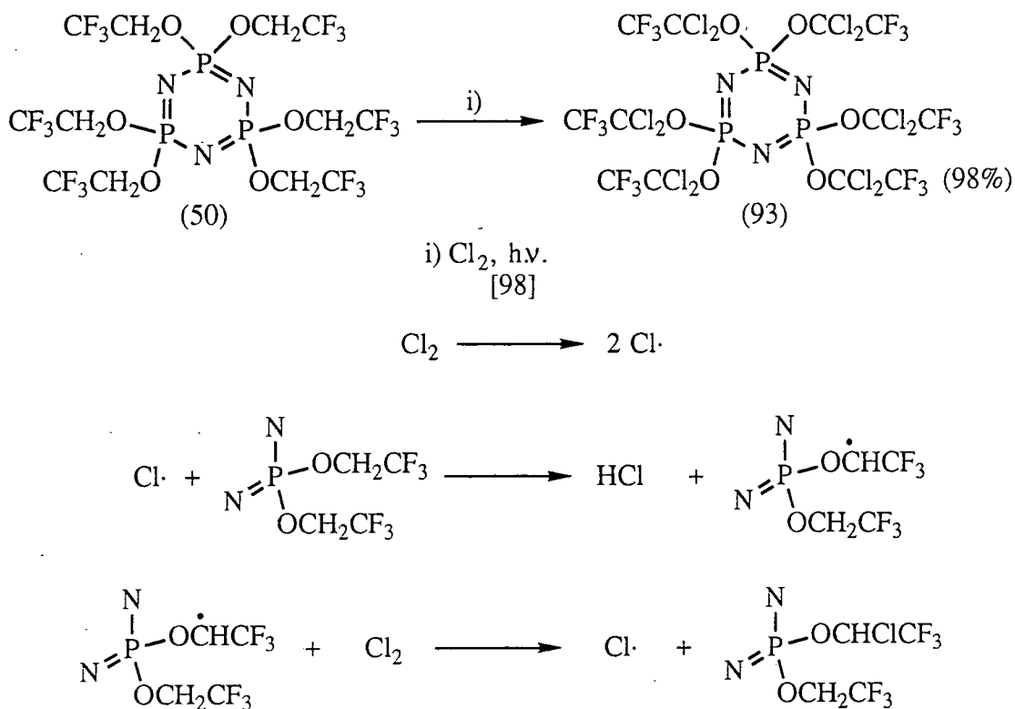
Scheme 12. Mechanism of the chlorination
