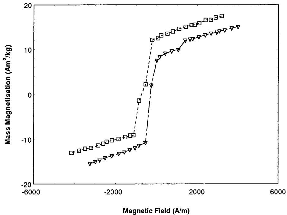
Fig.4.2a Low field region of a magnetic ink with a concentration of 0.9 \text{ kg/m}^3
