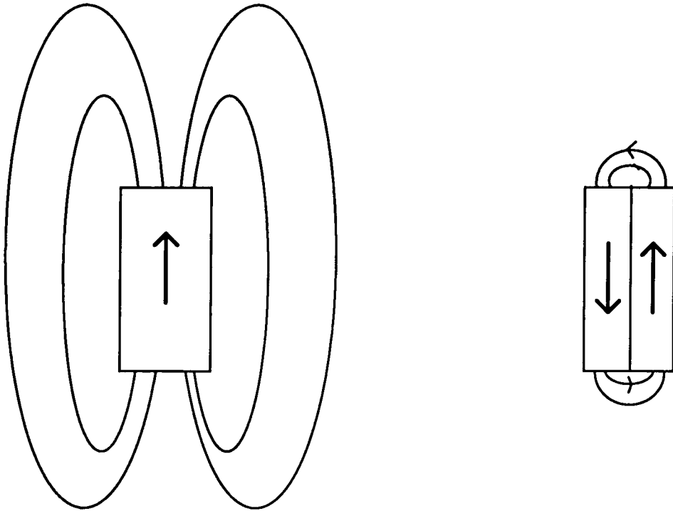
Fig.1.3 Diagram showing the formation of domains and the lowering of the demagnetising energy due to domain formation
