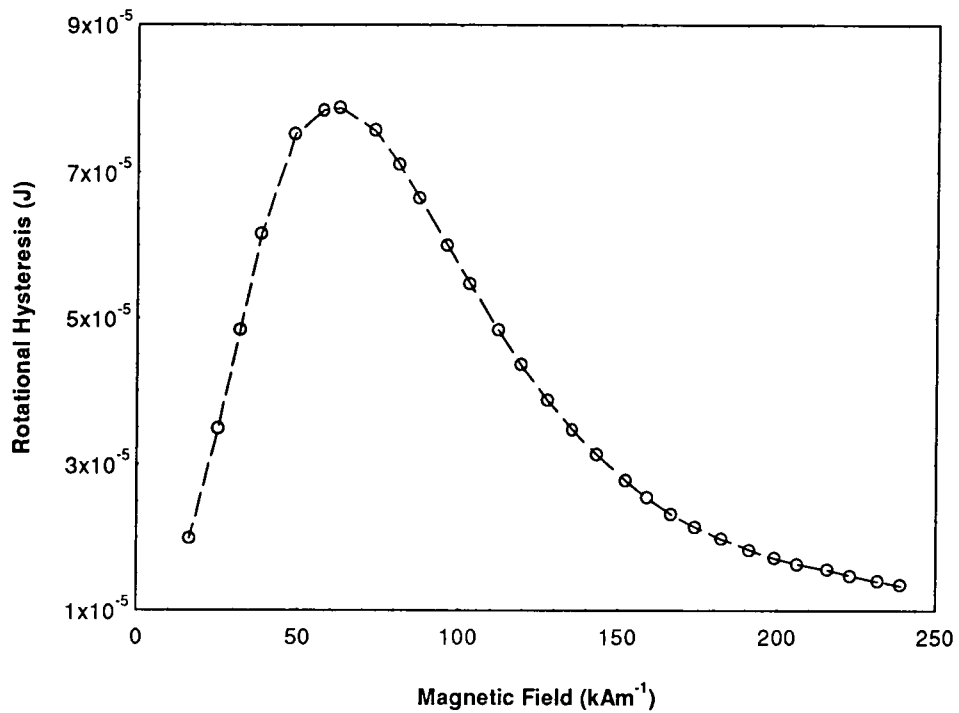
Fig.4.20 Rotational hysteresis as a function of magnetic field for a potted ink sample.
