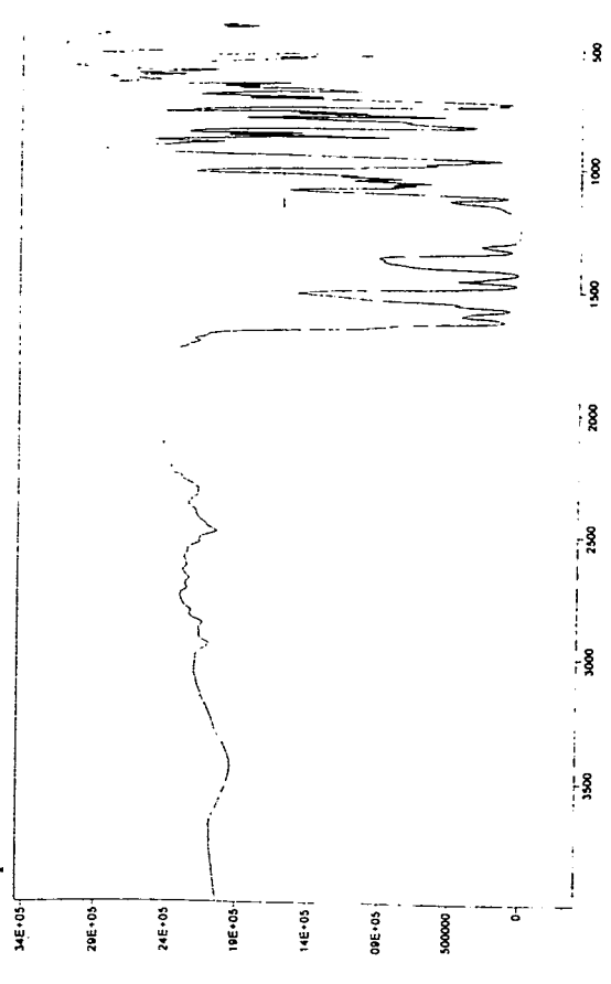
Spectrum No. 4
