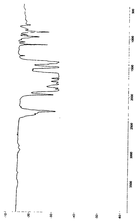
Spectrum No. 2
