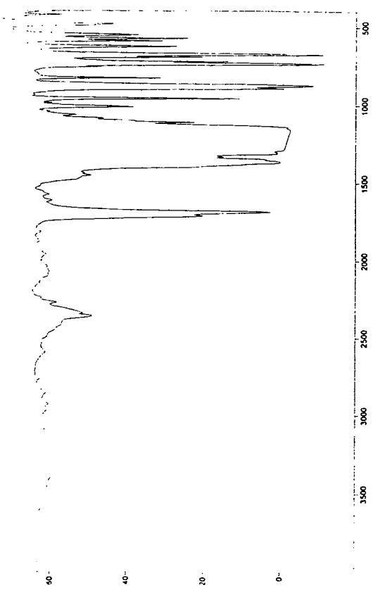
Spectrum No. 1
