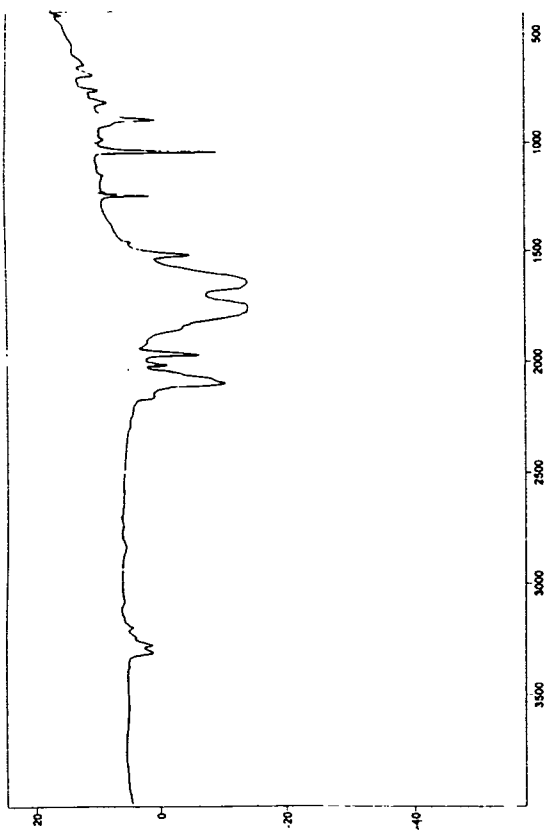
Spectrum No. 26
