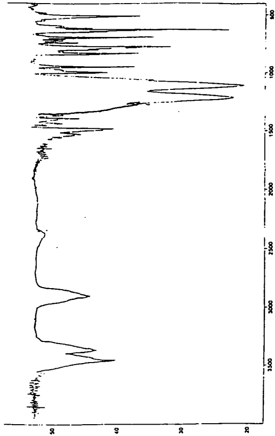
Spectrum No. 16
