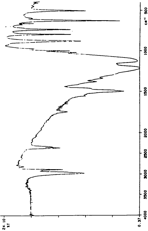
Spectrum No. 14
