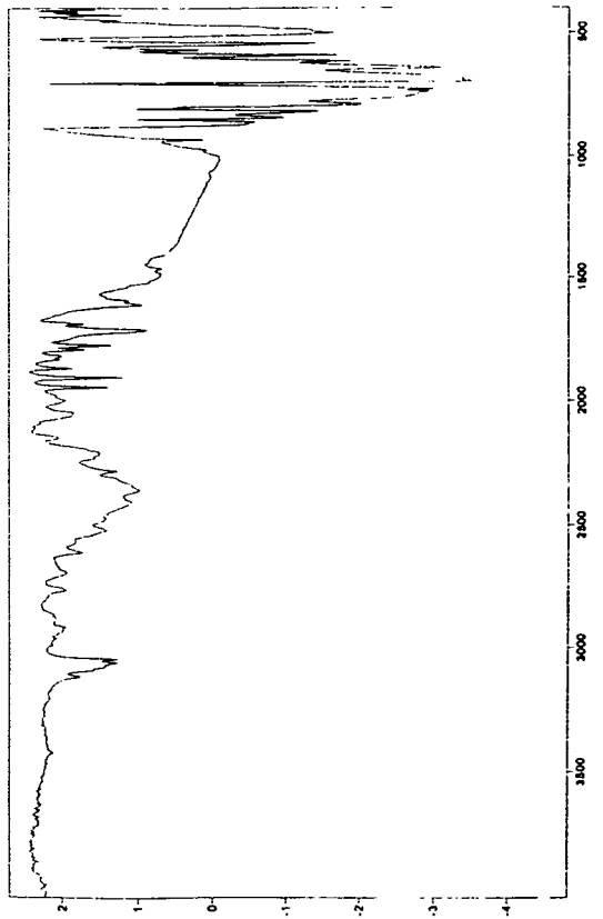
Spectrum No. 8
