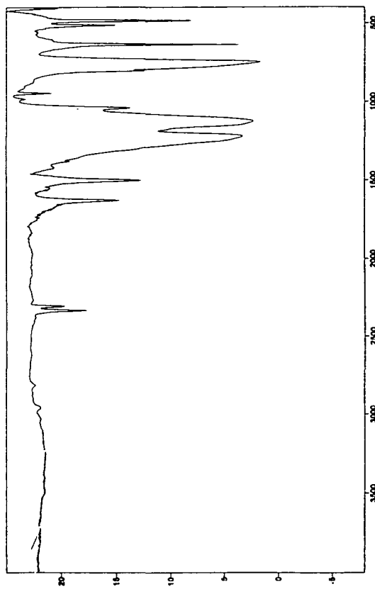
Spectrum No. 19
