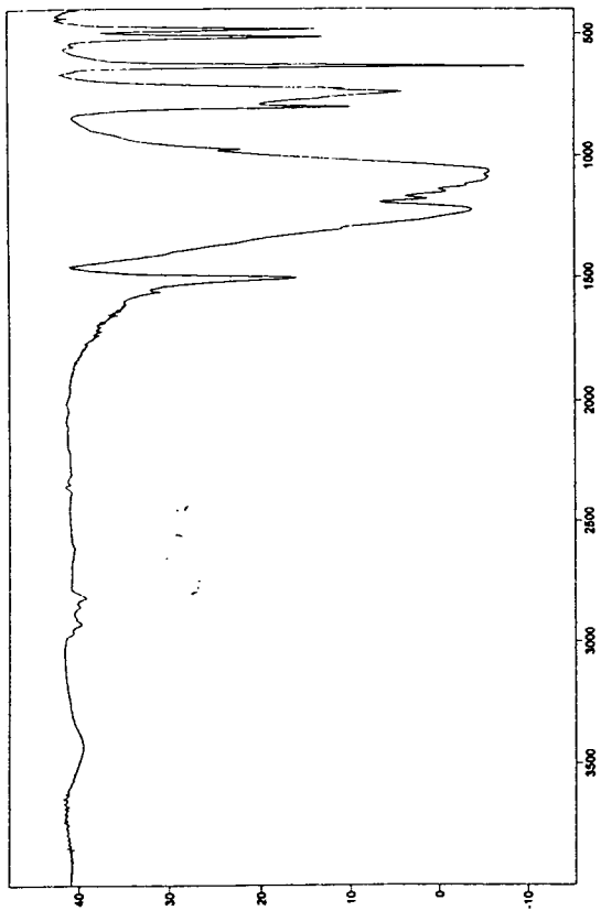
Spectrum No. 13
