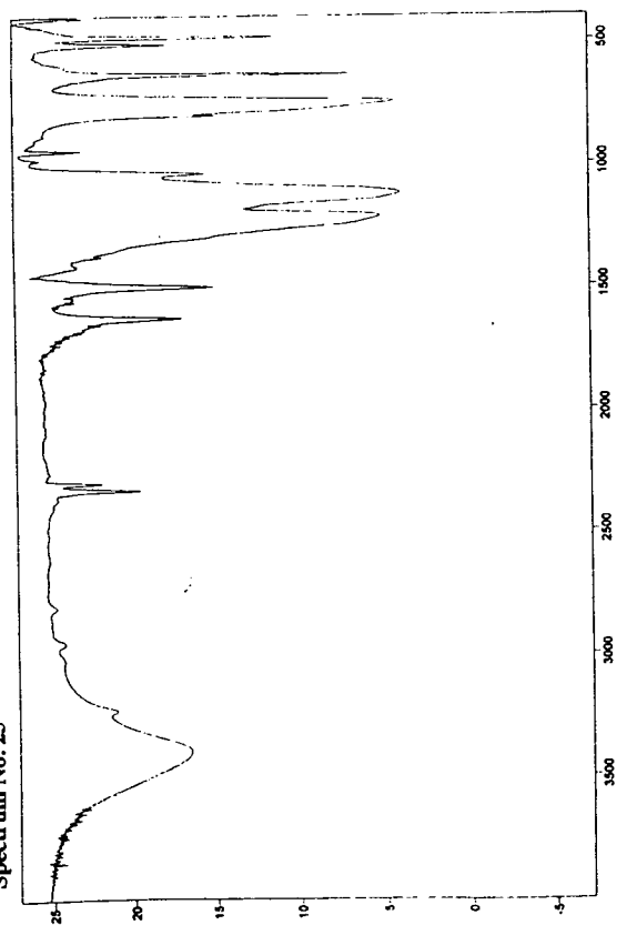
Spectrum No. 25
