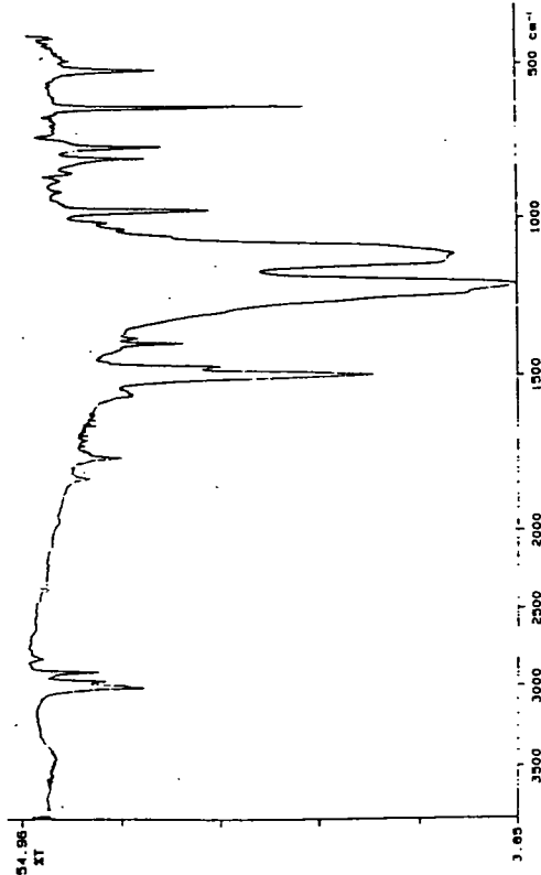
Spectrum No. 15
