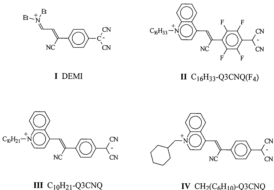
Figure 6.1 Molecular Structures of the zwitterionic chromophores investigated.
