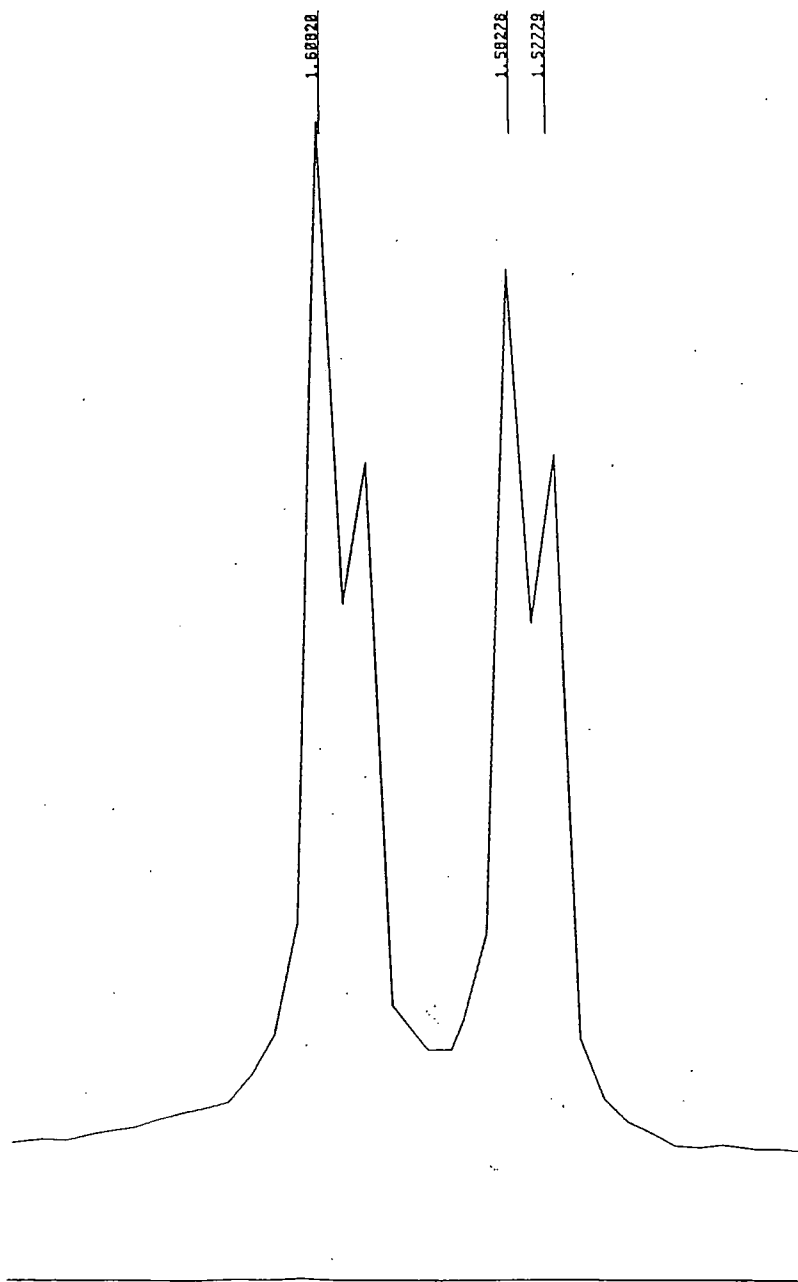
Figure 44. The ^1\text{H} NMR spectrum between (0-2 ppm) of (145) in the presence of optically active amide (2) .
