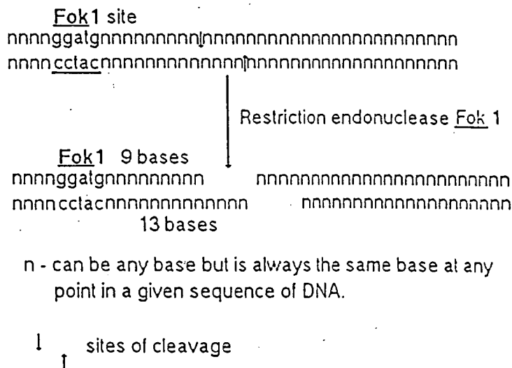
Figure 4. Nature of the cleavage produced by the restriction endonuclease Fok I .
