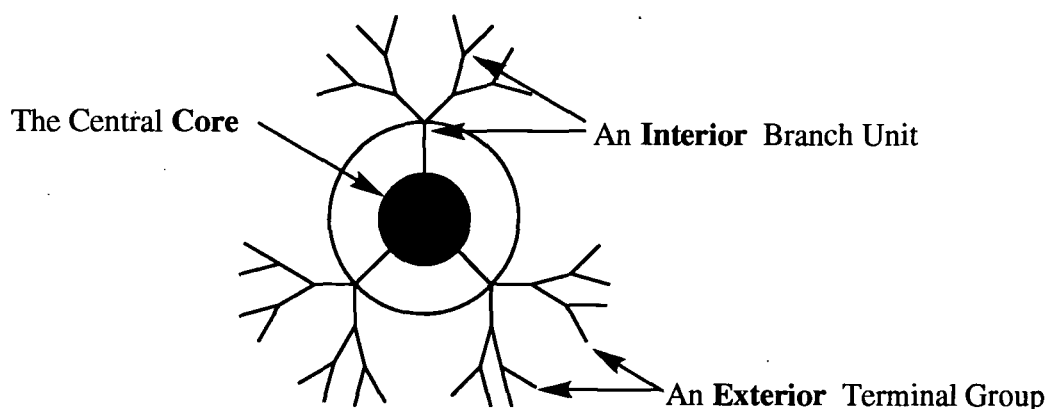
Figure 1.2.2 The Architectural Regions of a Dendrimer
