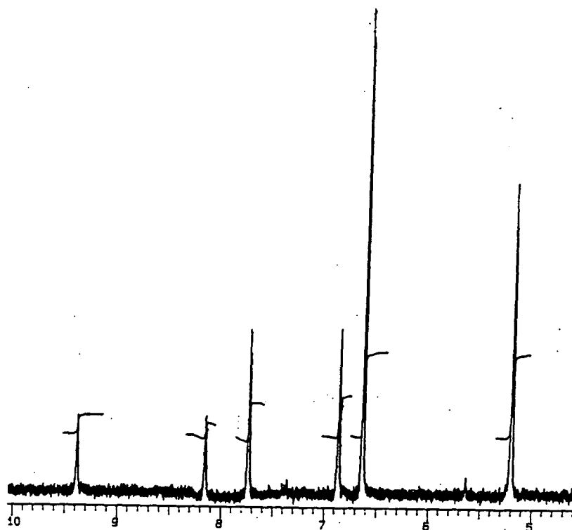
Figure 2.3.1 ^1\text{H} NMR Spectrum of Second Generation Silyl Ether 52
