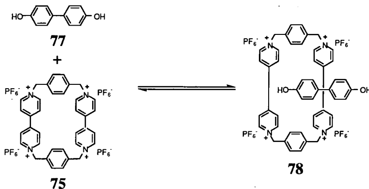
Scheme 4.2.2 Model [2]Pseudorotaxane 78
