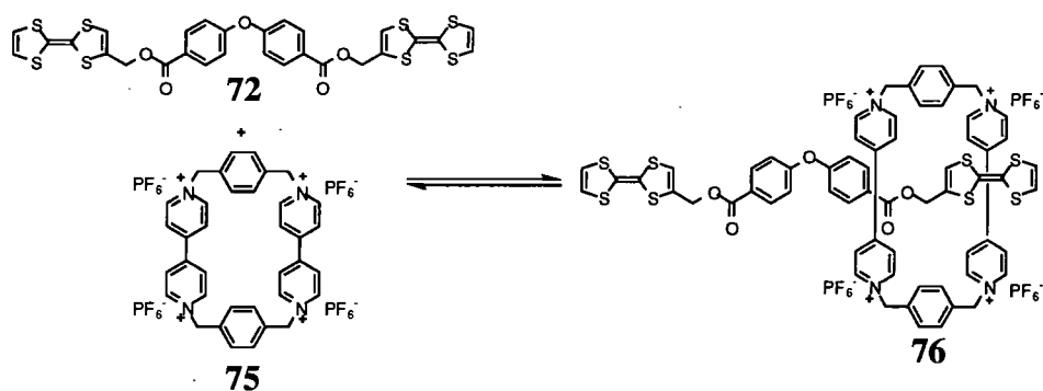
Scheme 4.2.1 Formation of [2]Pseudorotaxane 76
