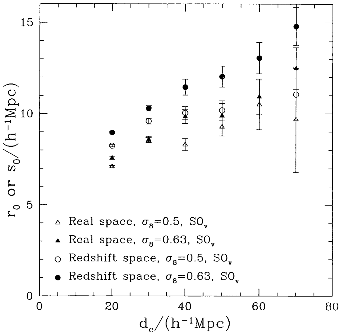
Figure 4.8: Variation of the redshift space correlation length, s_0 , with mean inter-cluster separation, d_c , for a selection of cluster catalogues. Data are for SO groups selected according to velocity dispersion. Open symbols show results for \sigma_8 = 0.5 and filled symbols for \sigma_8 = 0.63 . Circles represent our redshift space results and triangles the corresponding real space results from Fig. 4.6 which are included for comparison.
