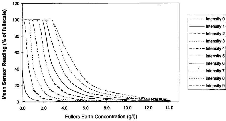
Figure 4.11. Mean sensor reading vs fuller's earth concentration. (gap = 40mm).
