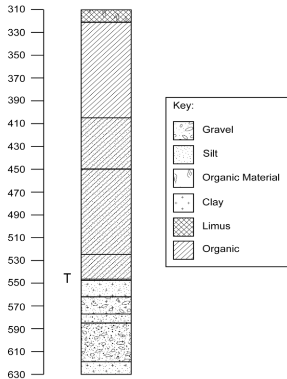
Figure 5.4: Sediment stratigraphy for the section of the SK1-1 core analysed for diatom and tephra analyses, showing the composition of each sediment layer. T represents the position of the sampled tephra layer within the analysed core section.
