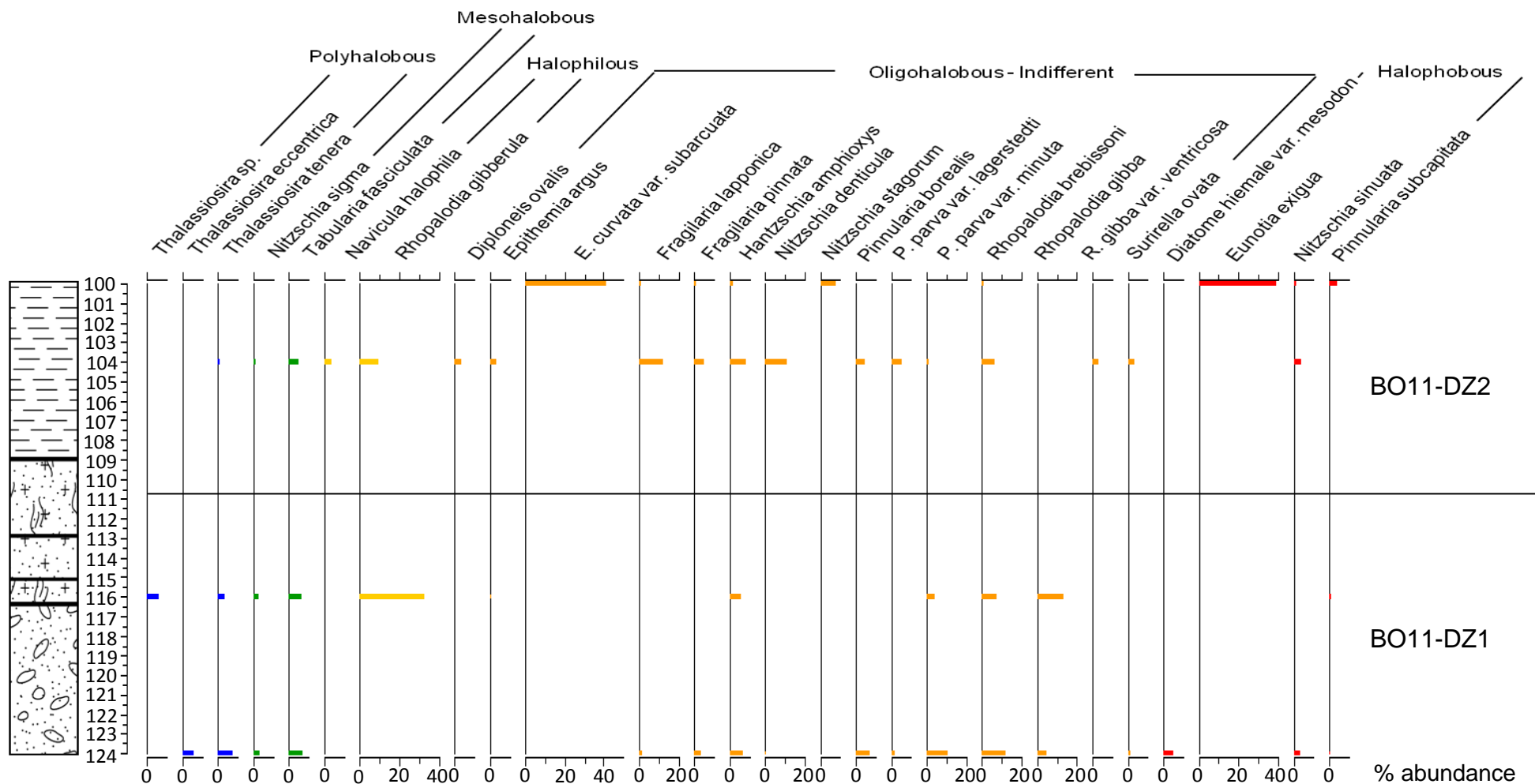
Figure 5.3: Diatom assemblage graph for the Borgarland 11 site, showing the transitional sequence. Key to sediments can be found in Fig. 5.1
