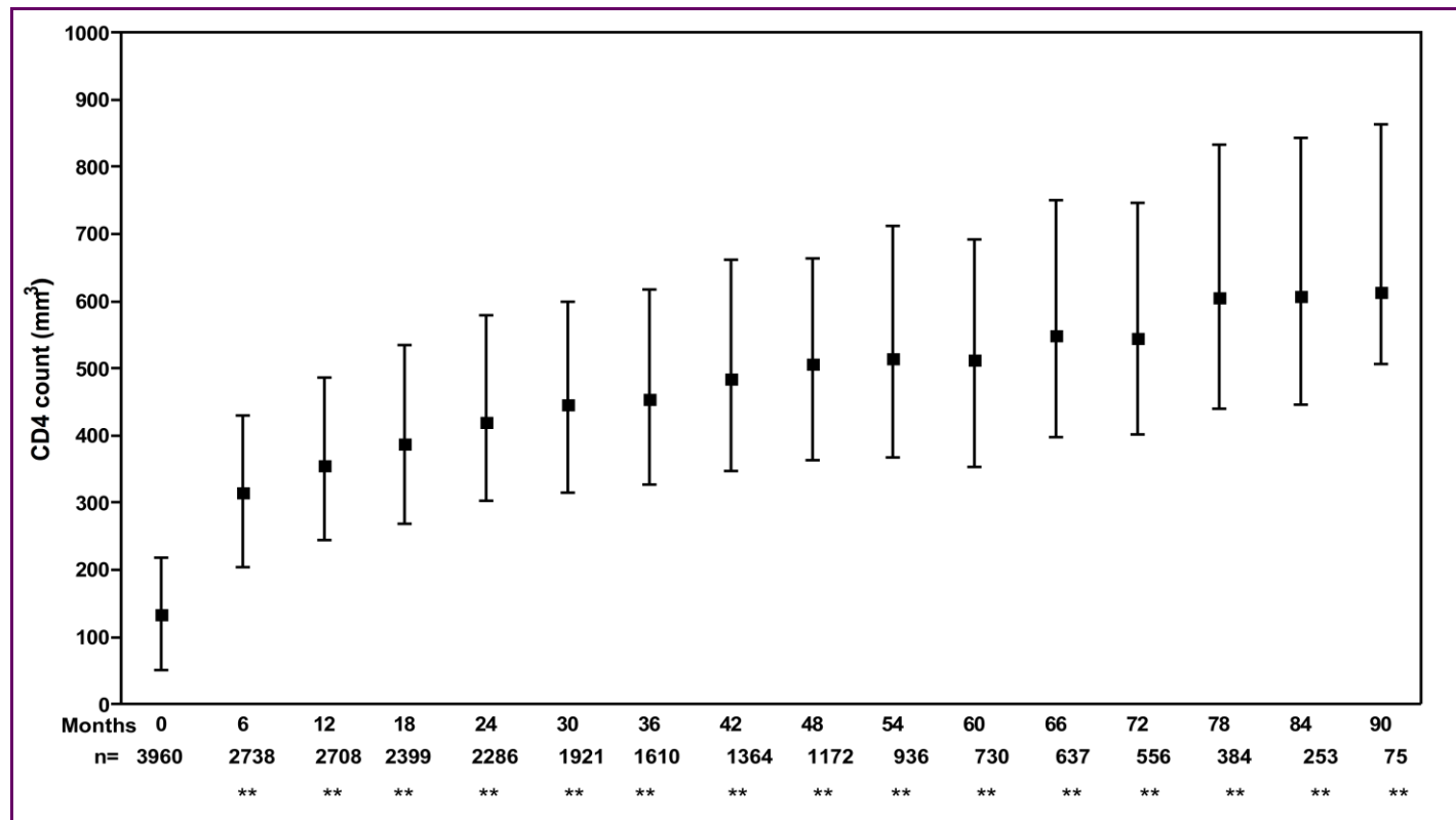
Figure 4.1. Changes in CD4 T-cell counts on cART. Each full square box represents the median, horizontal lines represent the Interquartile range and double asterixes indicate statistically significant difference obtained by pair-wise comparison of median with month 0 using the Mann-Whitney's U-test with p < 0.0001 representing a statistically significant difference.
