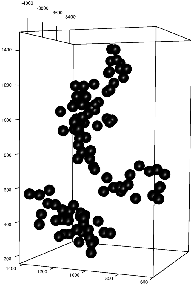
Figure 2. Snapshot from a visualization of both the new, Huger-LQG, and the CCLQG. The scales shown on the cuboid are proper sizes (Mpc) at the present epoch. The tick marks represent intervals of 200 Mpc. The Huger-LQG appears as the upper LQG. For comparison, the members of both are shown as spheres of radius 33.0 Mpc (half of the mean linkage for the Huger-LQG; the value for the CCLQG is 38.8 Mpc). For the Huger-LQG, note the dense, clumpy part followed by a change in orientation and a more filamentary part. The Huger-LQG and the CCLQG appear to be distinct entities.
