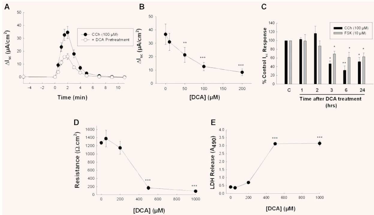
Fig. 2 Chronic exposure to low concentrations of DCA inhibits Cl - secretion across T 84 cells. (A) Monolayers of T 84 cells were exposed to bilateral DCA (50 μM) for 24 hrs and subsequent I sc responses to CCh (100 μM) were measured. (B) T 84 cell monolayers were exposed to increasing concentrations of DCA for 24 hrs after which I sc responses to CCh (100 μM) were measured ( n = 5). (C) Cells were exposed to DCA (50 μM) for varying periods after which I sc responses to CCh (100 μM; n = 4) or FSK (10 μM; n = 4) were measured. (D) Monolayers of T 84 cells were exposed to increasing concentrations of DCA for 24 hrs after which TER was measured ( n = 5). (E) Aliquots of supernatants from cells exposed to DCA at varying concentrations for 24 hrs were analysed for LDH. Data are expressed as sample absorbance at 490 nm ( n = 3). * P < 0.05; ** P < 0.01; *** P < 0.001.
