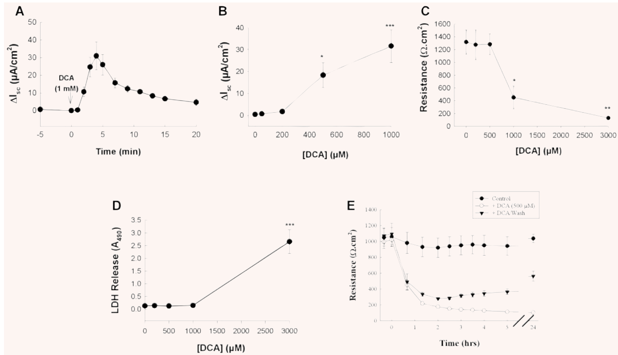
Fig. 1 Acute exposure to high concentrations of DCA stimulates Cl^- secretion across T_{84} cells. (A) Voltage-clamped monolayers of T_{84} cells were bilaterally exposed to DCA (1 mM) and I_{sc} responses were recorded ( n = 5 ). (B) Voltage-clamped T_{84} cells were exposed to increasing concentrations of bilateral DCA and maximal I_{sc} responses were measured ( n = 5 ). (C) Monolayers of T_{84} cells were exposed to increasing concentrations of DCA for 20 min after which TER was measured ( n = 3 ). (D) Aliquots of supernatants from cells exposed to DCA at varying concentrations for 20 min were analysed for LDH release. Data are expressed as sample absorbance at 490 nm ( n = 3 ). (E) TER was measured across T_{84} cell monolayers exposed to 500 \mu M DCA (bilateral). In one set of monolayers DCA was removed after 40 min ( n = 4 ). * P < 0.05 ; ** P < 0.01 ; *** P < 0.001 .
