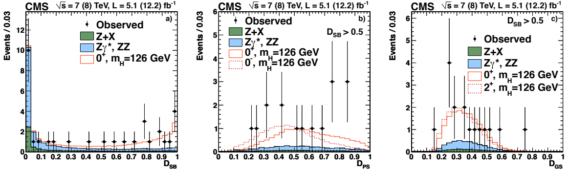
Figure 2: a) Observed distribution of the D_{SB} (SM Higgs boson versus background) discriminant compared with the background and signal expectations. b) Observed distribution of D_{PS} ( J^P = 0^- versus J^P = 0^+ ) compared with expectation, for D_{SB} > 0.5 . c) Observed distribution of D_{CS} ( J^P = 2^+ versus J^P = 0^+ ) compared with expectation, for D_{SB} > 0.5 . Points represent the observed data, shaded histograms represent the background, and the open histogram represent the expectation for a 126 GeV boson with the indicated spin-parity, produced at the SM Higgs boson rate.
