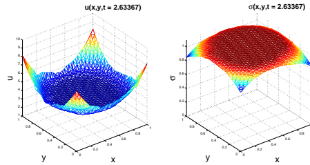
FIGURE 6. Snapshot for the 'hi-fi' scheme.
