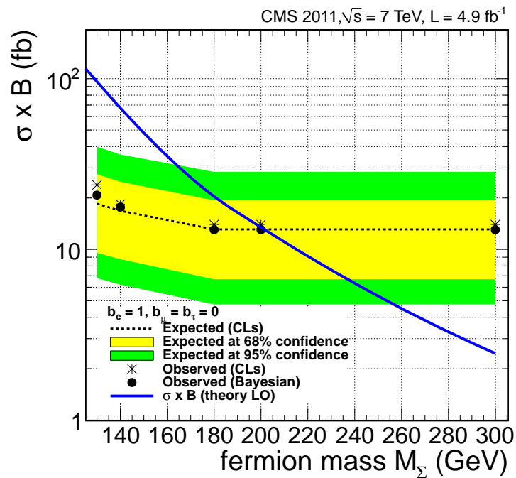
Figure 5: The expected (dashed line) and observed (black points) exclusion limits at 95% confidence level on \sigma\mathcal{B} as a function of the fermion mass M_\Sigma , assuming b_e = 1, b_\mu = 0, b_\tau = 0 (eS) for the signal. The solid (blue) curve represents the predictions of the LO type III seesaw models. The light (yellow) and dark (green) shaded areas represent, respectively, the 1 standard deviation (68% CL) and 2 standard deviations (95% CL) limits on the expected results obtained from MC pseudo-experiments, which reflect the combined statistical and systematic uncertainties of the SM contributions. The asterisks and the black points show, respectively, the observed limits computed following a frequentist method based on the CLs criterion and a Bayesian approach.
