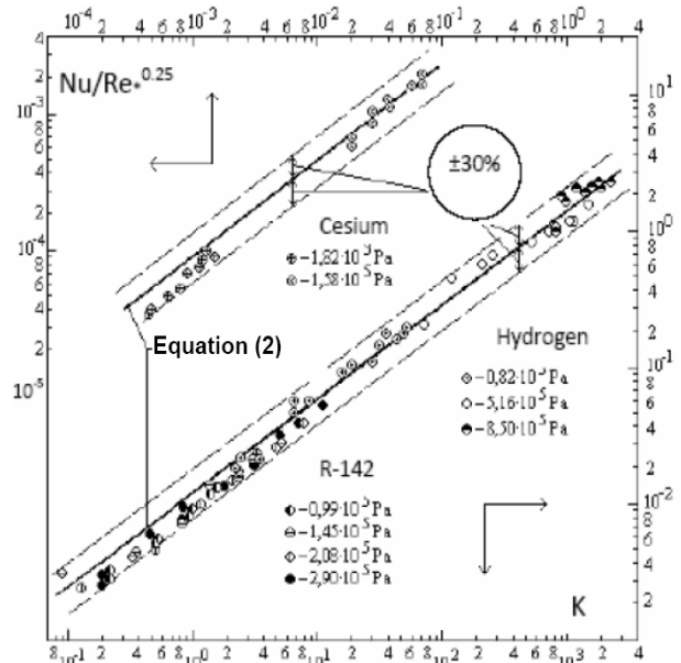
Fig. 2. Correlation of experimental data on developed boiling of cesium (Subbotin et al., 1976), R 142 (Danilova, 1976) and hydrogen (Grigoriev et al., 1975) on commercial surfaces ( \rho_0 = 5 \mu\text{m} ).
