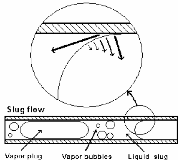
Fig. 4. Leading vapor plug in near to critical (pre-crisis) regime.
