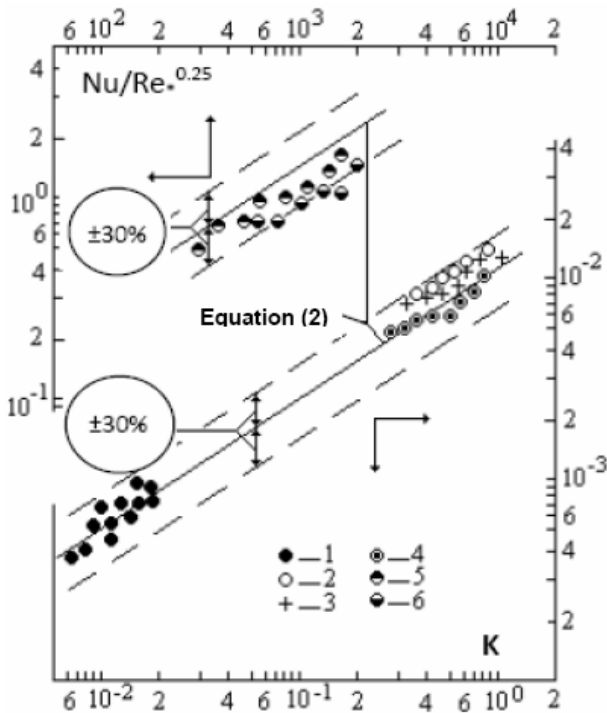
Fig. 1. Correlation of experimental data on developed boiling on the surfaces with the known values of \rho_0 : 1 – sodium (Marto and Rosenow, 1966), \rho_0 = 50 \mu\text{m} ; 2-4 – water (Shoukri and Judd, 1975), \rho_0 = 5 \mu\text{m} ; 5 – R 12 (Chumak et al, 1979), \rho_0 = 86 \mu\text{m} ; 6 - R 22 (Chumak et al., 1979), \rho_0 = 86 \mu\text{m} .
