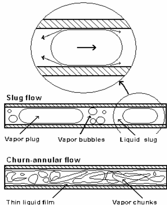
Fig. 4. Dominant flow regimes during boiling of Fluorinert FC-77 in microchannel with the width 100 \mu\text{m} (Harirchian and Garimella, 2009).
