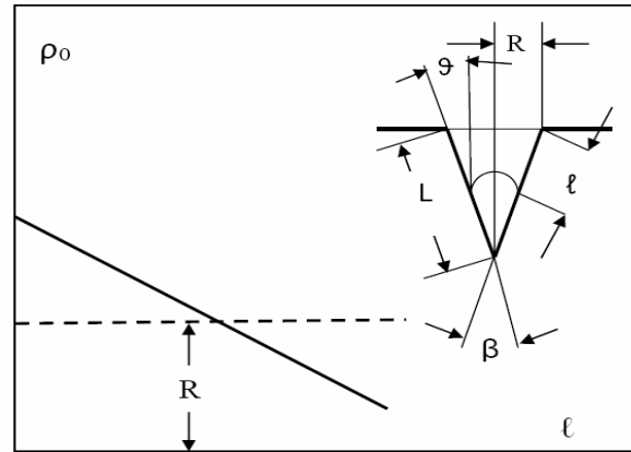
Fig. 3. Dependence of effective radius on a degree of wetting of nucleation site by liquid phase in the case \beta/2 > \theta .
