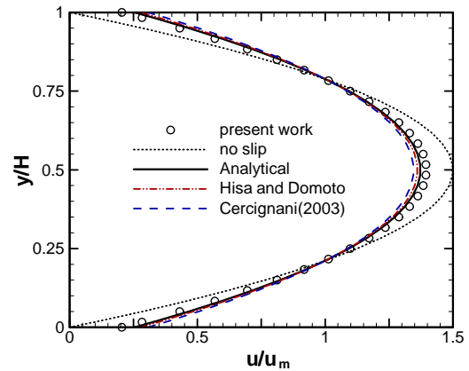
Fig. 7. Slip and no-slip velocities at the middle section of the channel for Kn=0.06 .
