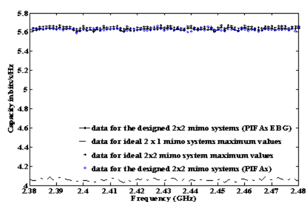
Figure 5: Measured capacity of PIFAs with and without EBG.
