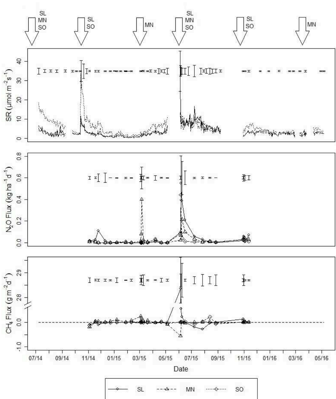
Figure 3 Soil Respiration (SR, \mu\text{mol m}^{-2} \text{s}^{-1} ), \text{N}_2\text{O} ( \text{kg ha}^{-1} \text{d}^{-1} ) and \text{CH}_4 ( \text{g m}^{-2} \text{d}^{-1} ) fluxes. Bars represent the differences between back-transformed least square means confidence intervals (0.5%÷95%). The arrows on top indicate the fertilization events.
