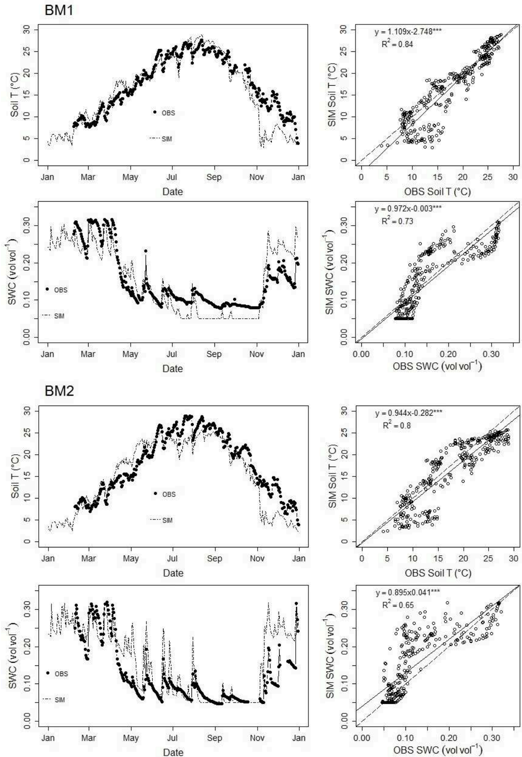
Figure 3 Calibration (BM1) and validation (BM2) results for Soil T (Soil Temperature, °C) and SWC at 0.03 m (Soil Water Content, \text{m}^3\text{m}^{-3} ) and relation between observed (OBS) and simulated (SIM) data. (***: P < 0.001 )
