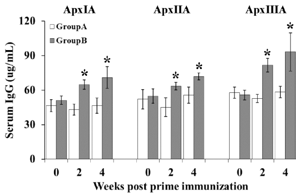
FIGURE 2. Serum IgG concentrations against the individual C-terminal fragments in piglets immunized intramuscularly with the combination vaccine. Data are presented as the mean of all piglets in each group and error bars show the standard deviation (SD). Asterisks indicate significant differences between the values of the inoculated group B and those of the control group A (* p < 0.05 )
