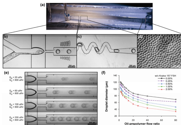
Fig. 2. Microencapsulation device. (a) Overview of device showing two aqueous input streams (red, blue) dispersed by shear flow from an oil stream into droplets that mix (purple) and travel down the UV-exposure channel. (b) Prepolymer (2× concentrated) and a cell suspension meet and flow into a 60 μm droplet generating nozzle. Vertical columns on either side of the channel provide visual references (50-100 μm below, 100-150 μm above) for real-time adjustment of droplet size. See Supporting Information for movie. (c) Droplets pass through a bumpy serpentine mixer section to thoroughly disperse cells in prepolymer and are then polymerized by UV irradiation from a curing lamp. (d) Microtissues collected from the device (6000/min) are spherical and monodisperse. (e) Microtissue size is controlled by the relative flow rates of the combined aqueous phase ( Q_P ) and the continuous oil phase ( Q_O ), and increases with prepolymer:oil flow ratio. (f) Adding small amounts of Krytox 157 FSH fluorosurfactant into the oil decreased droplet diameter at all flow ratios, allowing higher prepolymer flow rates for a given microtissue size.
