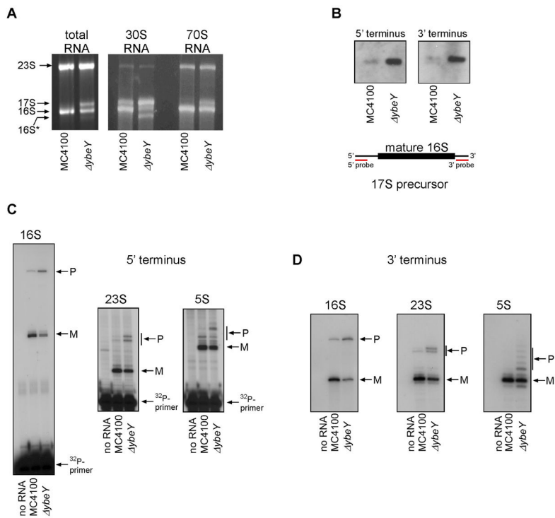
Figure 3. Analysis of rRNA from E. coli MC4100 and the \Delta ybeY mutant. (A) Total RNA isolated from whole cells, 30S ribosomal subunits and 70S ribosomes from MC4100 and the \Delta ybeY mutant. The positions of 23S, 17S, 16S and 16S* rRNAs are indicated based on their mobility. (B) Northern blot analysis using probes directed against the 5'- and 3'-termini of 17S rRNA. Equal amounts of total RNA from MC4100 and the \Delta ybeY mutant were used. The locations of the probes are shown in the diagram below the blots. (C, D) Primer extension and site-specific RNase H cleavage assays to map the 5'- and 3'-termini of 16S, 23S and 5S rRNAs from MC4100 and the \Delta ybeY mutant. "P" and "M" indicate the location of bands corresponding to precursor and mature forms of the rRNA, respectively. Annotation of the positions of the 5' and 3'-termini of 16S, 23S and 5S rRNAs, mature and precursor species, were based on previous observations (Li et al. , 1999b). Total RNA was prepared from MC4100 and the \Delta ybeY mutant strains as described in the Methods section.
