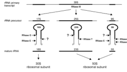
Figure 1. Steps in the processing of rRNA in E. coli . All enzymes indicated are endonucleases with the exception of RNase T that generates mature 3' termini by trimming the rRNA precursors.
