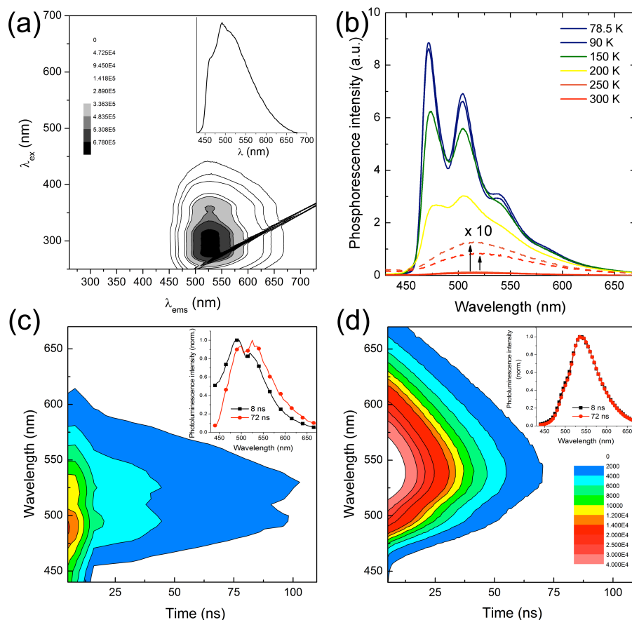
Figure 2. (a) Photoluminescence action spectrum of ZIrF (298 K). Inset figure is phosphorescence spectrum at \lambda_{\text{ex}} = 340 nm. (b) Phosphorescence spectra at various temperatures ( \lambda_{\text{ex}} = 340 nm). Room temperature time-resolved emission spectra (TRES; \lambda_{\text{ex}} = 342 nm) of ZIrF in the (c) absence and (d) presence of zinc ion (3 equiv). Inset figures are normalized phosphorescence spectra at delay times of 8 and 72 ns. Identical depth scale is employed for (c) and (d). 10 \mu\text{M} ZIrF in air-equilibrated \text{CH}_3\text{CN} solutions were used for measurements.
