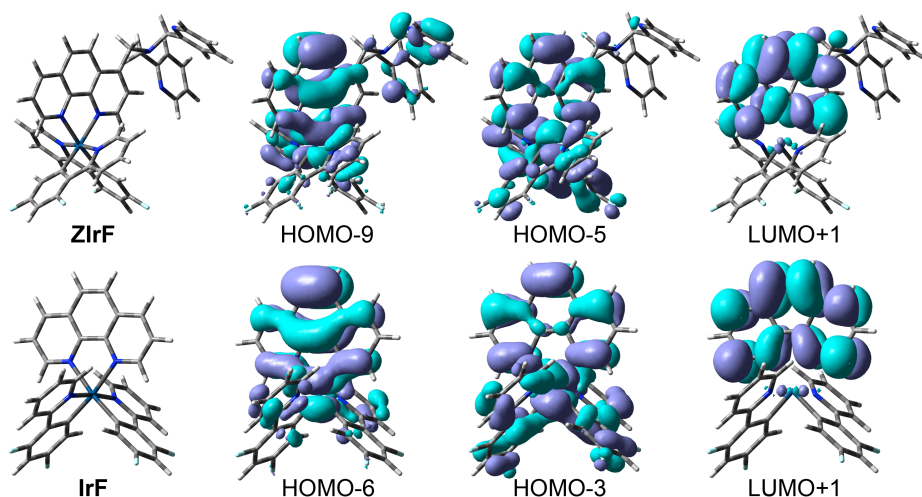
Figure 1. Calculated geometry and isosurface plot ( 0.04 e \text{ \AA}^{-3} ) of molecular orbitals that participate in the lowest energy triplet transition of ZIrF and IrF, as obtained from Gaussian 03.
