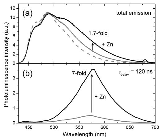
Figure 10. Time-gated acquisition of zinc-induced photoluminescence turn-on of ZIrF. (a) Total photoluminescence spectrum of an air-equilibrated pH 7.0 buffer solution (25 mM PIPES) containing ZIrF (10 \mu\text{M} ) and Acr + (2 \mu\text{M} ): Solid grey line, total photoluminescence spectrum; dashed grey line, fluorescence spectrum of Acr + (2 \mu\text{M} ); solid black line, after addition of ZnCl 2 (5 equiv). (b) Time-gated photoluminescence spectrum acquired after 120 ns delay: Grey line, zinc-free state; black line, after addition of ZnCl 2 (5 equiv). Excitation wavelength was 342 nm.
