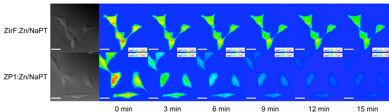
Figure 13. Comparison of photostability of ZIrF and ZP1. HeLa cells were incubated with Zn/NaPT, fixed, and then treated with either ZIrF or ZP1. Photoluminescence microscope images were taken every three min as the cells were illuminated by the excitation beam.
