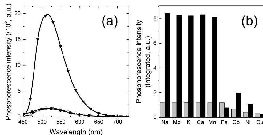
Figure 5. (a) Phosphorescence spectra of ZIrF showing reversible binding with zinc ions. Empty triangles, zinc-free solution; filled inverted triangles, in the presence of zinc ion (1 equiv); filled circles, after subsequent addition of TPEN (5 equiv). (b) Phosphorescent zinc selectivity of ZIrF. Grey bars, in the presence of metal ions; black bars, after subsequent addition of \text{ZnCl}_2 (1 equiv). \text{Na}^+ , \text{Mg}^{2+} , \text{K}^+ , and \text{Ca}^{2+} ions are 100 equiv. Other divalent metal ions are 1 equiv. Chloride salts were used. Conditions: 10 \mu\text{M} ZIrF in air-equilibrated pH 7.0 buffer (25 mM PIPES), \lambda_{\text{ex}} = 340 nm.
