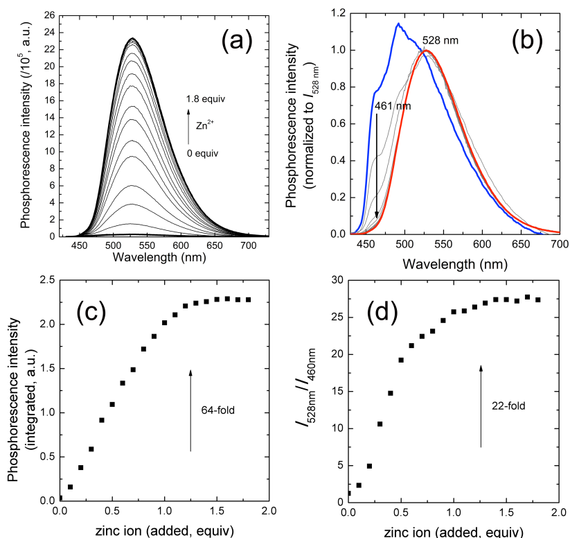
Figure 3. (a) Change in phosphorescence spectrum with increasing total zinc concentration. (b) Spectra shown in (a) are plotted to have same intensities at 528 nm: Blue line, zinc-free; red line, 1.8 equiv of zinc ion. (c) A titration isotherm plotting phosphorescence intensity as a function of amount of added zinc ion (equiv). (d) Change in phosphorescence intensity ratio at 528 nm vs 460 nm with various amount of added zinc ion. Condition: 10\ \mu\text{M} ZIrF in air-equilibrated \text{CH}_3\text{CN} , \lambda_{\text{ex}} = 340\ \text{nm} .
