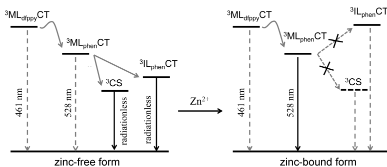
Figure 9. Schematic representation of the mechanism for zinc-induced phosphorescence turn-on of ZIrF ( \text{ML}_{\text{dfppy}}\text{CT} , metal-to-dfppy ligand charge-transfer transition state; \text{ML}_{\text{phen}}\text{CT} , metal-to-phen ligand charge-transfer transition state; CS, charge-separated state; \text{IL}_{\text{phen}}\text{CT} , intraligand charge-transfer transition state of phen ligand).
