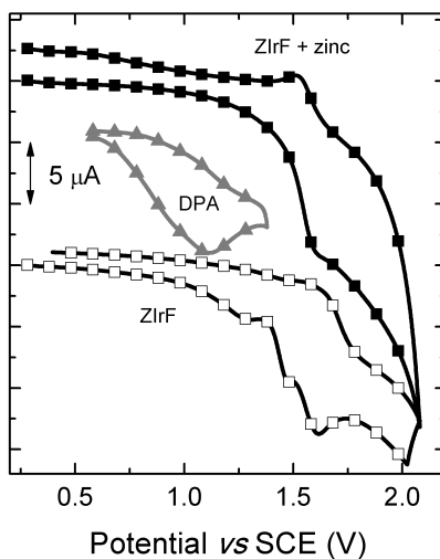
Figure 7. Cyclic voltammogram of ZIrF in the absence (empty squares) or presence (filled squares) of \text{Zn}(\text{ClO}_4)_2 (5 equiv). The cyclic voltammogram of di(2-picoyl)amine (DPA) is shown for comparison (filled triangles). Conditions: Scan rate = 100 mV/s; 1 mM in Ar-saturated \text{CH}_3\text{CN} containing \text{Bu}_4\text{NPF}_6 (0.1 M) supporting electrolyte; Pt wire counter and working electrodes; and the \text{Ag}/\text{AgNO}_3 couple for the reference electrode.
