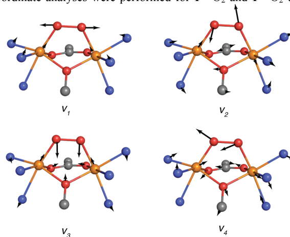
Fig. 2 Normal mode calculations for \mathbf{1}\cdot\text{O}_2 using the X-ray coordinates of [\text{Fe}_2(\mu\text{-O}_2)(\text{Ph-bimp})(\text{PhCO}_2)_2]^{2+} ( \mathbf{2}\cdot\text{O}_2 ), showing the vibrations that involve the \text{Fe}_2\text{O}_2 unit. The black arrows indicate the direction and relative degree of motion of the atoms to which they are attached. Color scheme: orange, iron; red, oxygen; blue, nitrogen; and gray, carbon.
