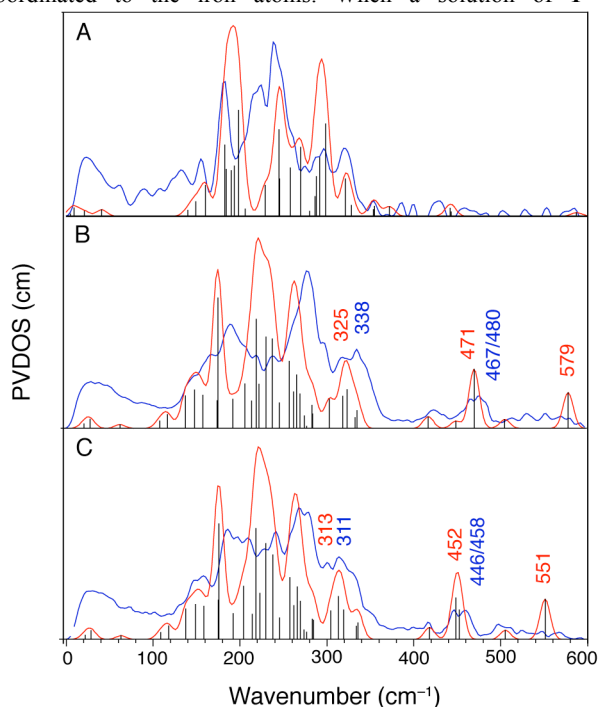
Fig. 1 ^{57}\text{Fe} partial vibrational density of states (PVDOS) for compounds 1 (A, 60 K, top), \mathbf{1}^{16}\text{O}_2 (B, 45 K, middle), and \mathbf{1}^{18}\text{O}_2 (C, 60 K, bottom) measured by NRVS. Panel A: Blue spectrum (selected peaks) = 182, 224, 240, 298, and 321\text{ cm}^{-1} . Red spectrum (selected peaks) = 192, 146, 195 \text{cm}^{-1} . Panel B: blue spectrum (selected peaks) = 190, 280, 338, 467, 480 \text{cm}^{-1} ; red spectrum (selected peaks) = 176, 225, 264, 325, 471, 579 \text{cm}^{-1} . Panel C: blue spectrum (selected peaks) = 186, 241, 281, 311, 446, 458 \text{cm}^{-1} ; red spectrum (selected peaks) = 175, 224, 262, 313, 452, 551 \text{cm}^{-1} . Color scheme: raw data in blue, empirical data fit in red, and individual eigenmode frequencies/intensities before broadening in black.
