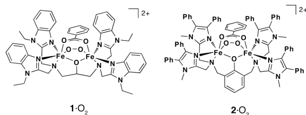
Chart 2 A proposed structure of [\text{Fe}_2(\mu\text{-O}_2)(N\text{-EtHPTB})(\text{PhCO}_2)]^{2+} ( 1\cdot\text{O}_2 , left). The benzoate ligand in 1\cdot\text{O}_2 may be coordinated in a terminal rather than bridging fashion. 37 The X-ray structure of [\text{Fe}_2(\mu\text{-O}_2)(\text{Ph-bimp})(\text{PhCO}_2)]^{2+} ( 2\cdot\text{O}_2 , right) has been determined. 39
