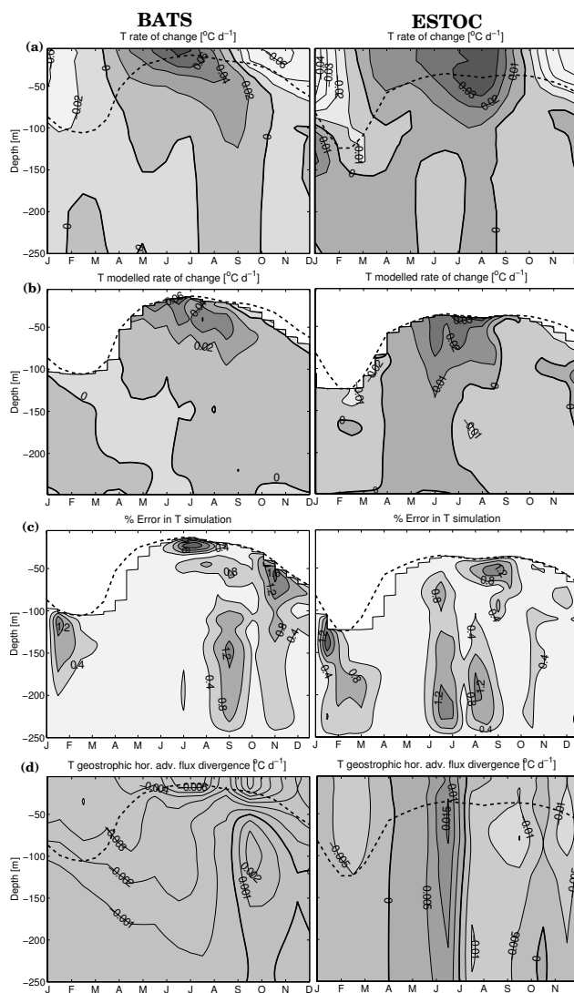
Fig. 5. (a) Observed and (b) simulated temperature rate of change, (c) errors in the simulated temperature seasonal cycle, and (d) geostrophic horizontal advection flux divergence at BATS and ESTOC. The black discontinuous line represents the mixed layer depth and the black thick line represents the zero rate of change isoline.
