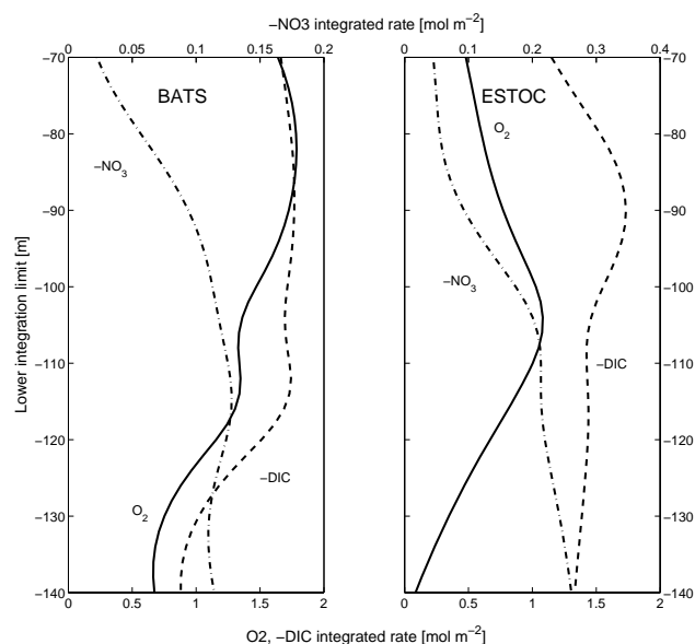
Fig. 7. Time and depth-integrated net production rates as a function of the lower limit used for the integration at BATS and ESTOC for oxygen (solid), DIC (dashed) and nitrate (dot-dashed).
