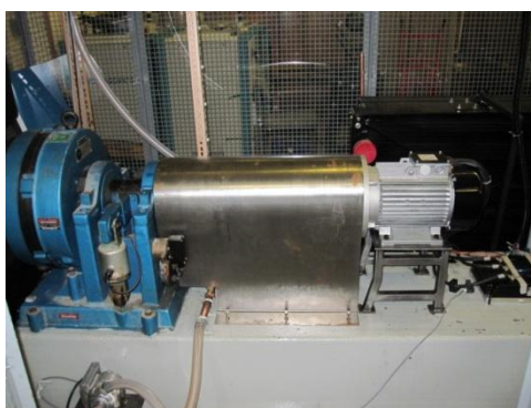
Fig. 2. Dynamometer hardware
