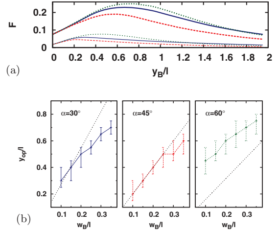
FIG. 3. (Color online) Wedge trap with the box at rest at x_B = 0 . (a) Fraction F of trapped atoms versus box positions y_B : \alpha = 30^\circ , w_B/l = 0.1 (solid blue line); \alpha = 45^\circ , w_B/l = 0.1 (dashed red line); \alpha = 60^\circ , w_B/l = 0.1 (dotted green line); \alpha = 30^\circ , w_B/l = 0.35 (thick solid blue line); \alpha = 45^\circ , w_B/l = 0.35 (thick dashed red line); \alpha = 60^\circ , w_B/l = 0.35 (thick dotted green line). (b) Optimal position y_{op} of the box at rest for different wedge angles (blue, red, respectively, green plus signs connected with lines), the black dots correspond to the straight line y_{op} = w_B(1 + \tan \alpha) / \tan \alpha ; see text for more details. t_f/\tau = 20 , E_B/E_i = 0.1 .
