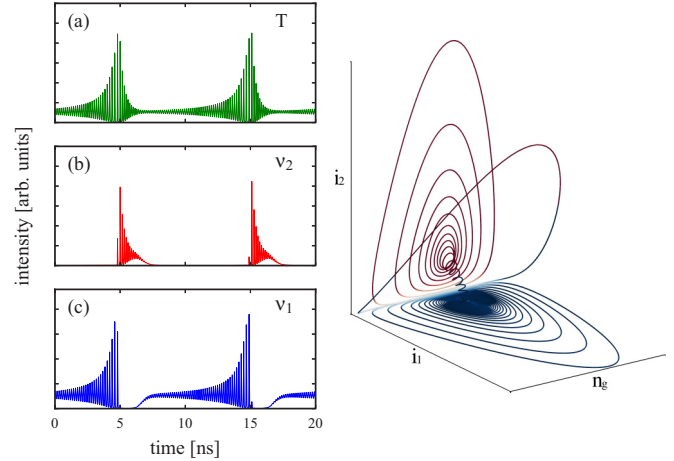
FIG. 9. (Color online) Left: Simulated intensity time traces. (a) Total intensity. (b) Long-wavelength mode \nu_2 . (c) Short-wavelength mode \nu_1 . Right: Phase-space diagram.
