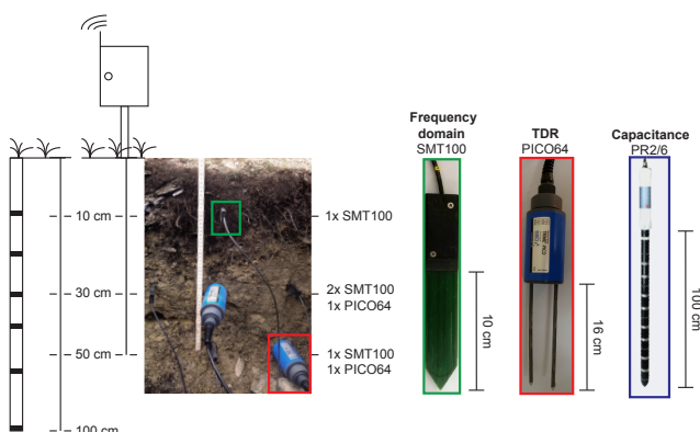
Figure 2. Instrumentation of the standard SOMOMOUNT station.
