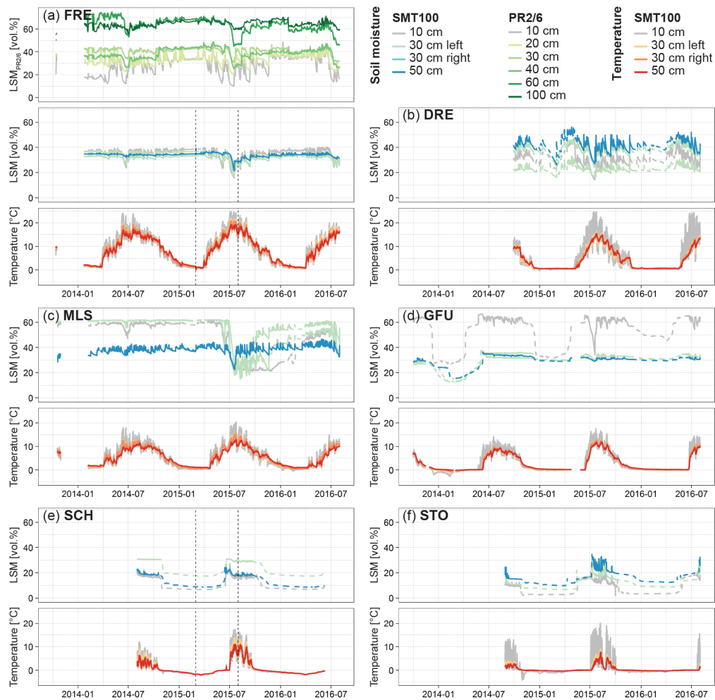
Figure 6. SMT100 measured LSM (upper panel) and ground temperatures (lower panel) at each SOMOMOUNT station (a–f). At FRE the uppermost panel displays the PR2/6 measured LSM. The vertical dotted lines at FRE and SCH indicate the period analysed in Fig. 7. The dashed LSM lines represent the soil moisture measurements taken when the ground temperature was below 1 °C.
