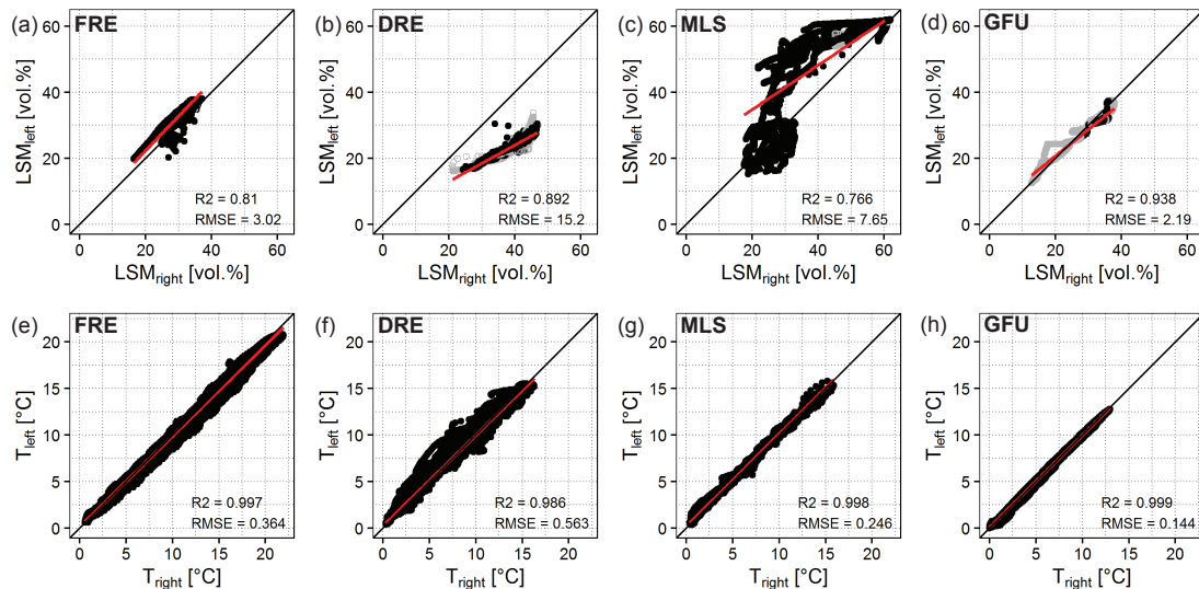
Figure 4. Comparison of measured LSM (upper row) and ground temperature (lower row) from both SMT100 sensors at 30 cm depth using the linear calibration at FRE (a, e), DRE (b, f), MLS (c, g) and GFU (d, h). The hollow grey points represent LSM measurements taken when the ground temperature was below 1 °C.
