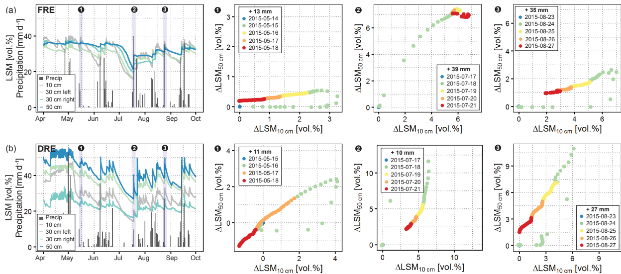
Figure 11. Moisture orbit at FRE (a) and DRE (b) for three precipitation events in 2015. The LSM values are hourly means and expressed as the change of absolute value compared to the first measurement (first day at 23:00). The daily precipitation sums recorded at the beginning of each event are indicated.
