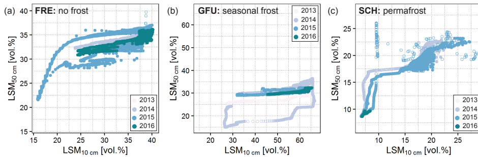
Figure 9. Moisture orbits at FRE (a), GFU (b) and SCH (c) for the consecutive monitoring years (January 2014–August 2016 at FRE, August 2013–August 2016 at GFU and August 2014–June 2016 at SCH). The hollow circles represent LSM measurements taken when the temperature was below 1 °C at 10 cm.
