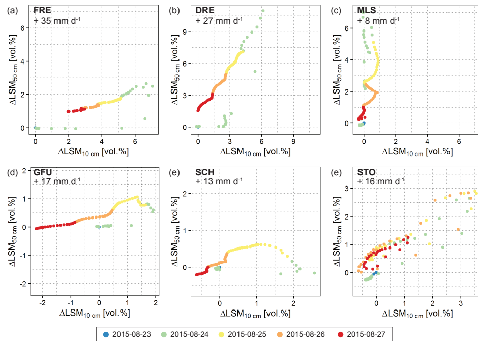
Figure 10. Moisture orbit at each SOMOMOUNT station for one precipitation event between the 23 and the 27 August 2015. The LSM values are given as hourly mean and expressed as the change of absolute value compared to the first measurement (23 August at 23:00). The daily precipitation sums recorded (FRE, DRE and MLS) and extrapolated (GFU, SCH and STO) for the 24 August are indicated.
