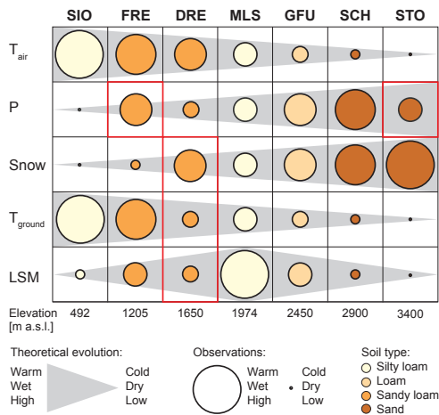
Figure 13. Generalized schematics of the evolution of air temperature, precipitation, snow duration, ground temperature and LSM with elevation. The circles represent the observations from 2015 (see Fig. 12), the grey area the expected theoretical evolution and the colour scale the soil type. The mismatches between model and observations are highlighted in red.
