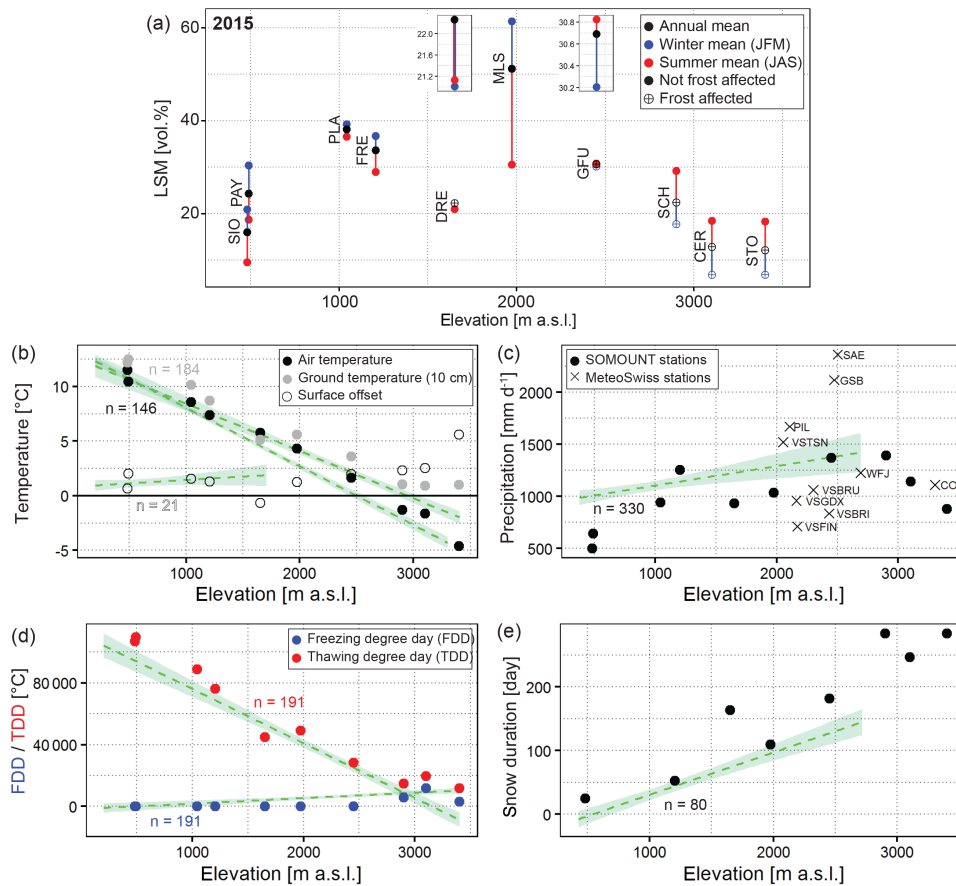
Figure 12. Elevation dependency of the winter, summer and annual mean LSM at 30 cm depth (a), air, ground temperature and surface offset (ground minus air temperature) at 10 cm (b), annual precipitation sum including selected SwissMetNet stations for comparison (see Fig. 1) (c), freezing and thawing degree days (calculated from ground temperatures at 10 cm) (d) and snow duration (calculated from ground temperature at 10 cm using the method described in Staub and Delaloye, 2017) (e) during the year 2015. The LSM values for SIO, PAY and PLA are part of the SwissSMEX network (Mittelbach and Seneviratne, 2012). Due to missing data at 30 cm, the LSM shown for PAY and PLA was measured at 50 and 20 cm at CER. The dashed green lines illustrate the linear regression based on all available SwissMetNet, PERMOS and IMIS stations in Switzerland (the numbers of station with complete data series in 2015 are indicated) and the shaded areas represent the 99 % confidence intervals. The length of each regression line corresponds to the maximum elevation of the available stations.
