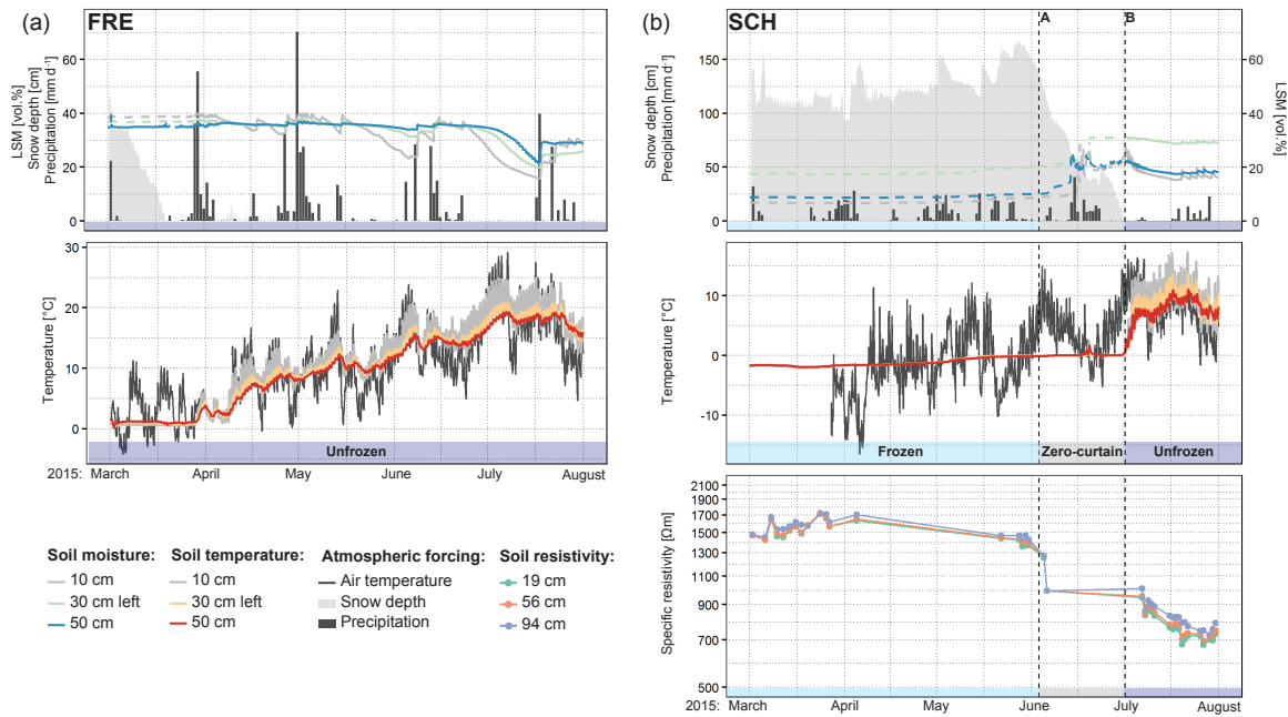
Figure 7. SMT100 measured LSM, ground temperature and soil resistivity at FRE (a) and SCH (b) from March to August 2015. In addition, daily air temperature, snow depth and precipitation sums are shown as well as the date of the transition between the different stages in the thermal evolution at SCH at 10 cm (dashed lines A and B; see text for details). The dashed LSM lines represent the soil moisture measurements taken when the ground temperature was below 1 °C.
