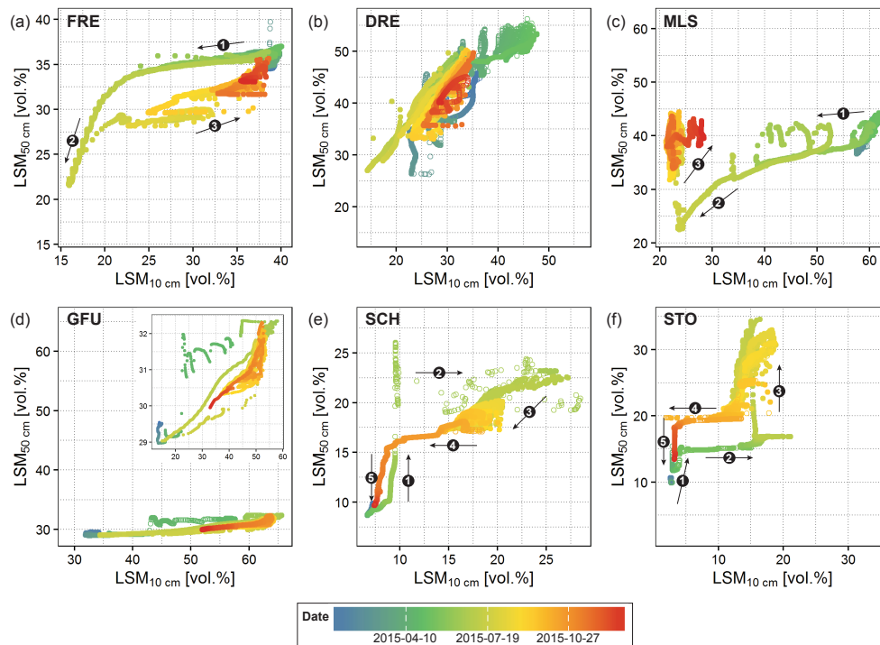
Figure 8. Moisture orbit at each SOMOMOUNT station from the 1 January to the 31 December 2015. The numbered arrows indicate the most important stages at each station as well as the sense of the evolution. The hollow circles represent LSM measurements taken when the temperature was below 1^{\circ}\text{C} at 10 cm.
