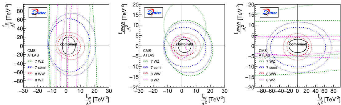
Figure 1. Results of the TGV analysis from LHC Run I. We show all two-dimensional profile likelihoods in the three-dimensional parameter space at 95% CL (2dof) for the individual channels as well as their combination.
