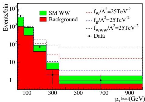
Figure 5. Leading p_{T,\ell} distribution for the 8 TeV ATLAS WW analysis [57]. The red histogram shows the ATLAS background estimate (excluding the SM WW prediction), while the green histogram shows the total SM prediction once WW processes are added. The observed events are shown as dots, with error bars accounting for the statistical uncertainty. The dashed lines indicate the effects of dimension-six Wilson coefficients.
