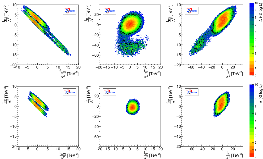
Figure 3. Correlated profile likelihood for sets of two Wilson coefficients. In the first row we include only LHC Run I Higgs data, including kinematic distributions, as shown in figure 11 of refs. [6, 7]. In the second row we add the Run I di-boson results probing anomalous TGV interactions (as well as the corresponding LEP results). The black points indicate -2 \log L = 5.99 . The corresponding one-dimensional profile likelihoods can be found in figure 4.
