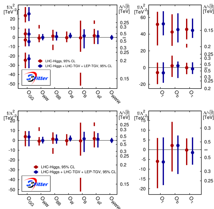
Figure 4. Allowed 95% CL ranges for individual Wilson coefficients f_x/\Lambda^2 from a one-dimensional profile likelihood. We show results from Run I Higgs observables only (red bars) and for a combined Higgs plus TGV analysis (blue). For the upper panels we allow for sign changes in the individual Yukawa couplings, while in the lower panel we fix their signs to the Standard Model one.
