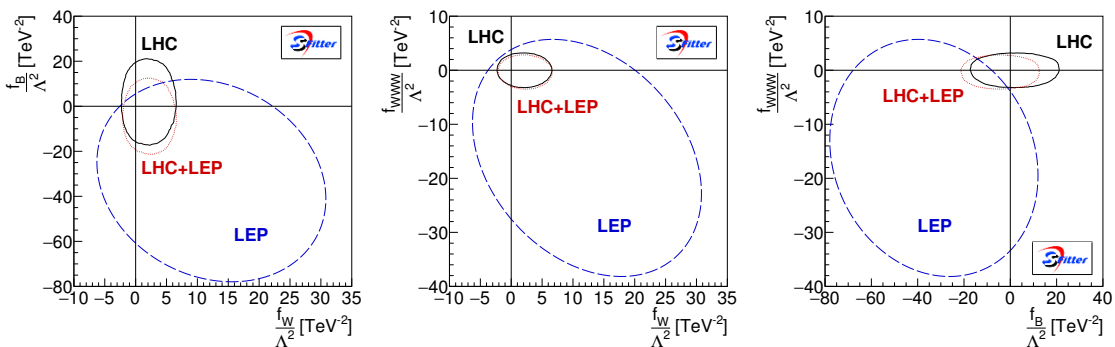
Figure 2. Results of the TGV analysis in terms of two-dimensional profile likelihoods from LHC Run I and from LEP [77]. We also show the statistical combination of both.
