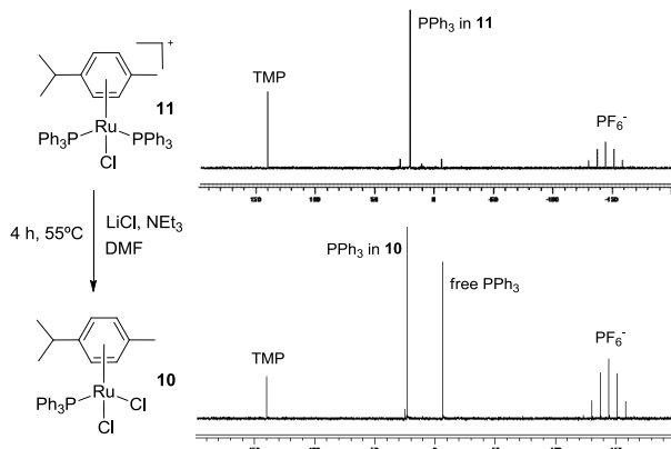
Figure 2. Schematic representation of the transformation of complex 11 to 10 (left) and ^{31}\text{P} NMR spectra of 11 (A) and of the reaction crude after heating 11 in the presence of LiCl and \text{NEt}_3 for 4 h at 55 °C (B).
