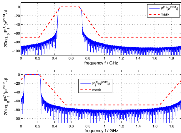
Fig. 11. Magnitude responses of stage 1 prototype filters for (top) US-1 configuration and (bottom) US-2 configuration.
