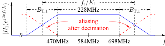
Fig. 8. Stage 1 (US-2) filter with passband width of 228MHz to capture upper portion TVWS spectrum, and transition bandwidth B_{T,1} .
