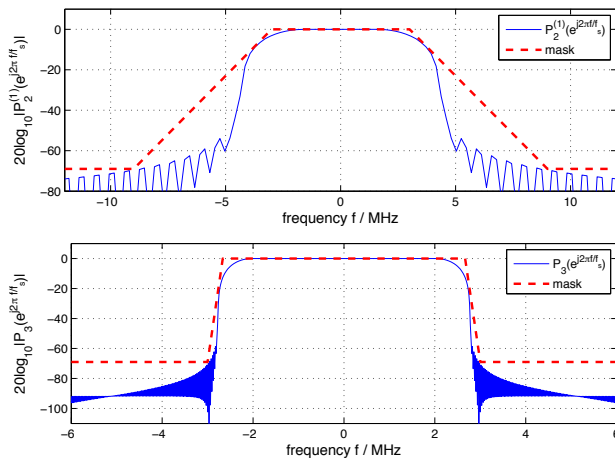
Fig. 12. Magnitude responses of stage 2 prototype filter (top) and stage 3 prototype filter (bottom) for US-1 and US-2 configurations.
