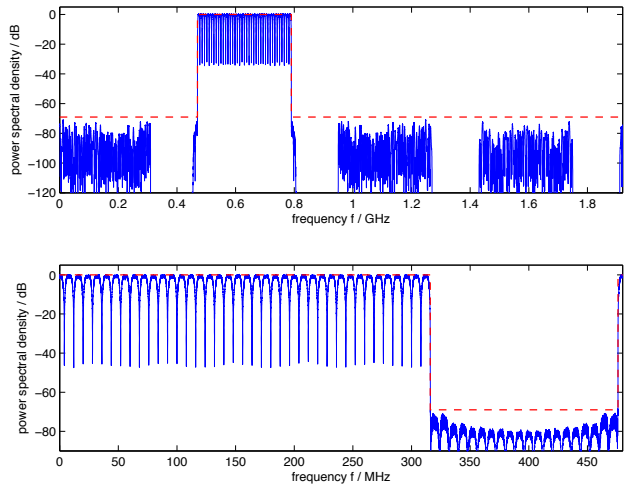
Fig. 10. Power spectral densities of stage 1 (top) and stage 2 (bottom) signals, with spectral masks indicated as dotted lines (UK).
