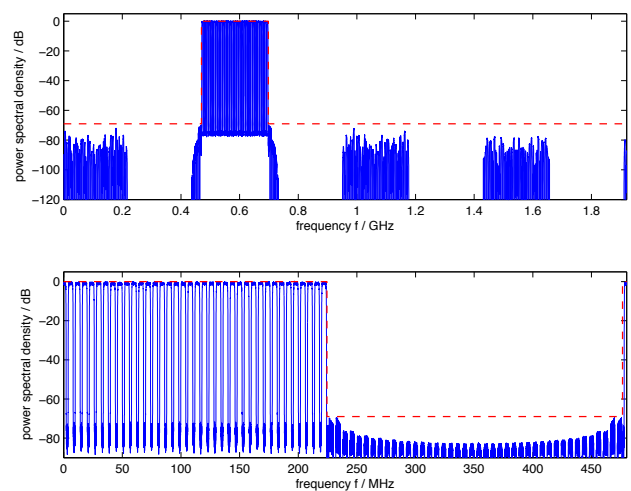
Fig. 14. Power spectral densities of stage 1 (top) and stage 2 (bottom) signals, with spectral masks indicated as dotted lines (US-2).
