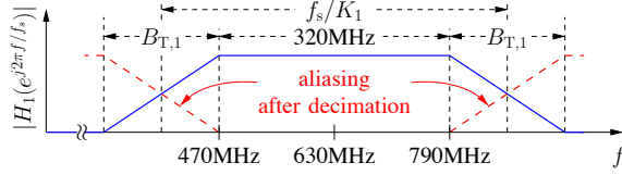
Fig. 3. Stage 1 (UK-1) filter characteristic with passband of 320MHz to capture the TVWS spectrum, and transition bandwidth B_{T,1} .
