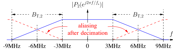
Fig. 7. Stage 2 (US-1,2) prototype filter with 6MHz passband width and decimation to 12MHz sampling rate.
