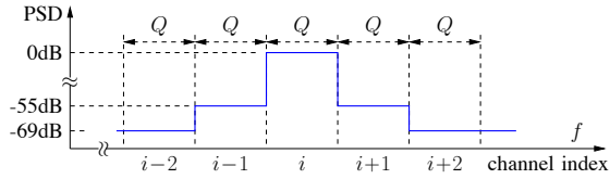
Fig. 1. Spectral mask defining permitted PSD levels in adjacent ( i \pm 1 ) and next-adjacent 8MHz TVWS channels ( i \pm 2 ) [1]. Q = \{6,8\} MHz according to configuration.
