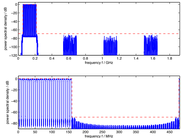
Fig. 13. Power spectral densities of stage 1 (top) and stage 2 (bottom) signals, with spectral masks indicated as dotted lines (US-1).
