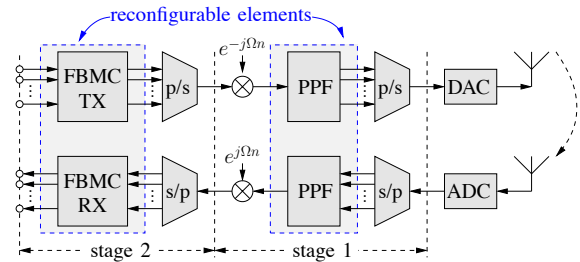
Fig. 2. Proposed reconfigurable TVWS filter bank transmitter (above) and receiver (below) with a polyphase filter (PPF) in stage 1 and a FBMC modulator in stage 2.
