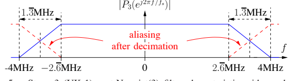
Fig. 5. Stage 3 (UK-1) root-Nyquist(3) filter characteristic with passband width of 5.3MHz and 16MHz sampling rate (for test purposes).
