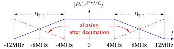
Fig. 4. Stage 2 (UK-1) filter characteristic with passband width of 8MHz and decimation to 16MHz sampling rate.
