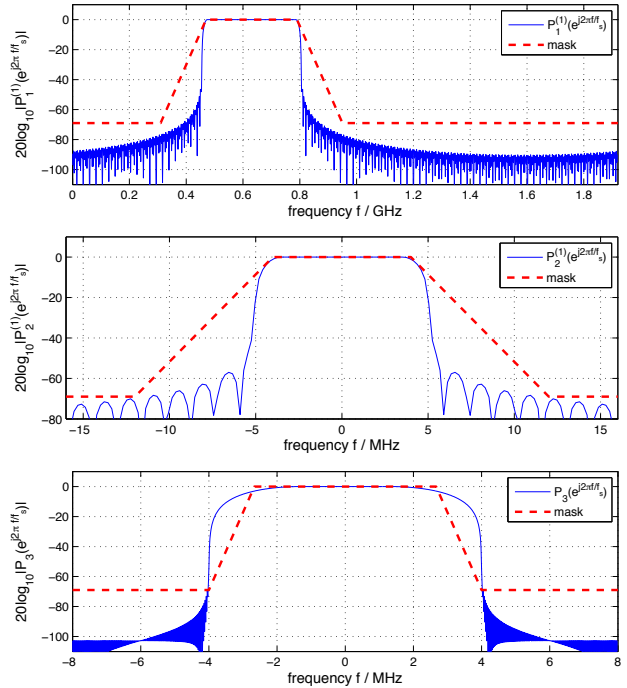
Fig. 9. Magnitude responses of (top) stage 1, (middle) 2, and (bottom) 3 prototype filters for UK configuration.
