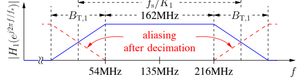
Fig. 6. Stage 1 (US-1) filter with passband width of 162MHz to capture lower portion TVWS spectrum, and transition bandwidth B_{T,1}
