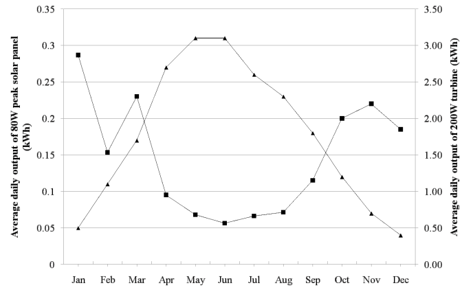
Fig. 3: Average daily power generation from a single 80 W PV module (▲) and a 200 W wind turbine (■) on the Isle of Tiree, Scotland, based on predicted solar irradiation data from the Photovoltaic Geographical Information System (PVGIS) [13] and averaged wind speeds measured at Tiree Airport between 2008 and 2010 with the wind turbine used for a “WindFi” base station.
