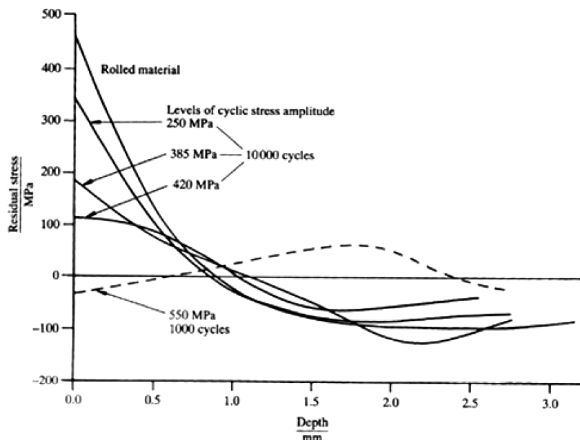
Fig. 2 The effect of vibration on residual stress induced by rolling (1 per cent reduction) in a sample of mild steel Note that there is no effect till the induced stress reaches 250 MPa
