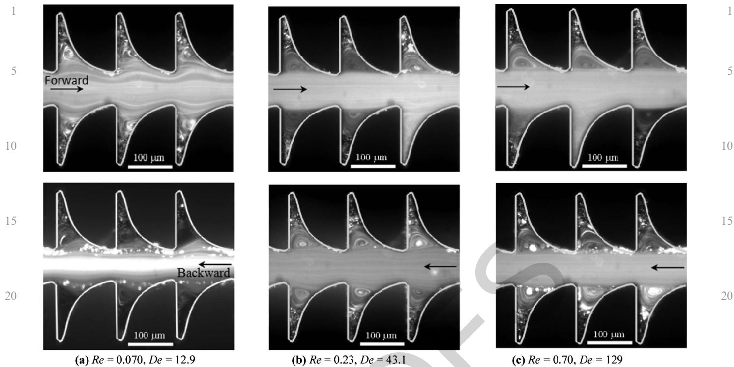
Fig. 3 Streak images of the viscoelastic fluid flow in rectifier B ( AR = 1.26 ; h = 88 \mu\text{m} ) at different flow rates.
