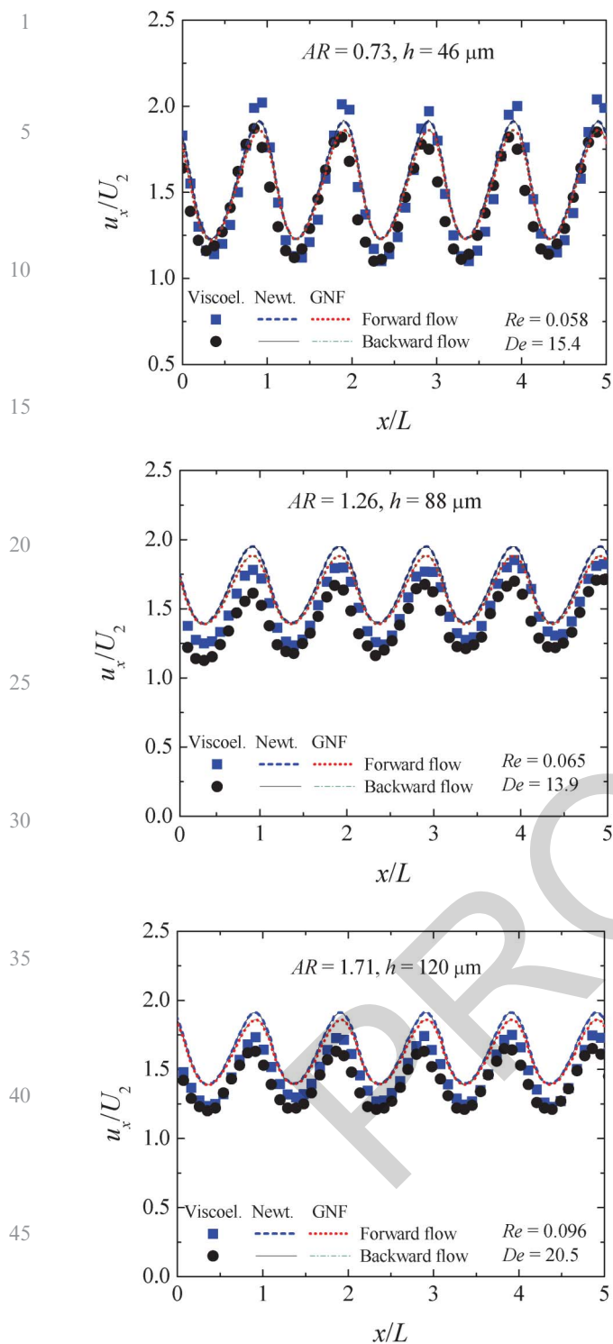
Fig. 5 Dimensionless axial velocity profiles along the centreline of the hyperbolic rectifiers with different aspect ratios under steady flow conditions. Symbols: experimental data for the viscoelastic fluid; lines: numerical predictions for a Newtonian and a generalized Newtonian fluid, described by the Carreau-Yasuda model, flowing at the same flow rate as the viscoelastic fluid.
