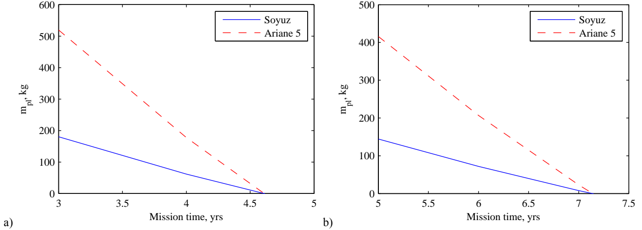
Figure 9. Payload mass ( m_{pl} ) as a function of the mission lifetime, for the pure SEP spacecraft (a) and the hybrid spacecraft (b).
