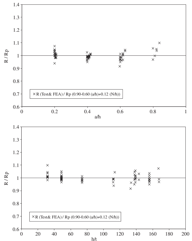
Fig. 9. Comparison of strength reduction factor for flanges unfastened condition under ETF loading condition.
