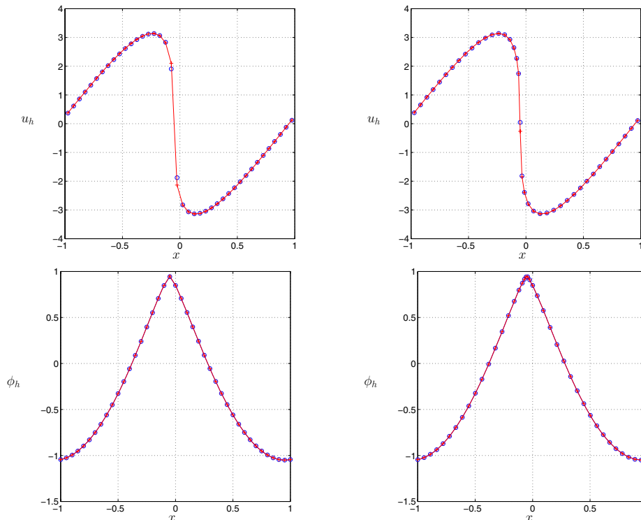
FIG. 1. DG numerical solution (o) and exact solution (+) obtained on a uniform stationary mesh (left) and on a moving mesh (right) at time t = 0.99/\pi^2 .
