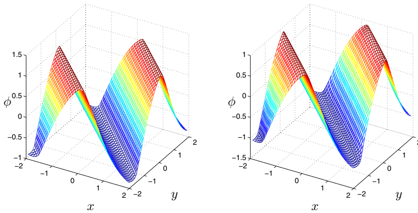
FIG. 13. Approximations of \phi at t = 1.5/\pi^2 using a uniform mesh (left) and adaptive moving mesh (right), where CFL = 0.05 and N = 40 , for Example 5.
