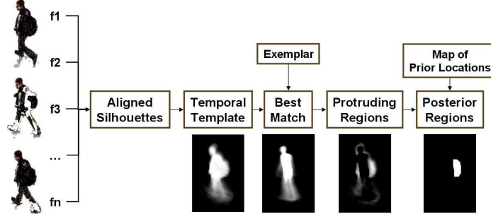
Fig. 1. All the frames in the the sequence are first aligned. The temporal template represents the frequency of each aligned pixel (relative to the median) being part of the foreground. The exemplar temporal template from a similar viewing angle is transformed (translation, scaling and rotation) to best match the generated temporal template. By comparing the temporal template to the best match, protruding regions are identified. MRF with a map of prior locations is used to decide on those pixels representing carried objects.
