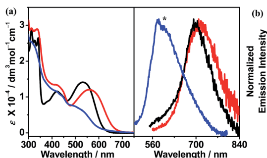
Fig. 3 (a) UV-vis absorption and (b) emission spectra ( [\text{Pt}] \approx 1 \times 10^{-5} \text{ M} ) of ( 1 ) 1 , ( 2 ) 2 and ( 3 ) mononuclear complex in \text{CH}_2\text{Cl}_2 at 298 K. (The asterisk indicates the instrumental artifact.)
