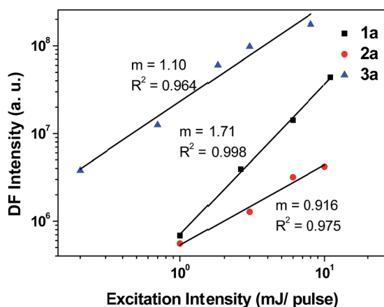
Fig. 12 Dependence of delayed fluorescence of 1a – 3a in 5 \times 10^{-5} M degassed \text{CH}_2\text{Cl}_2 with excitation power intensity. Emission intensity measured after a time delay of 1 \mu\text{s} . (Laser \lambda_{\text{exc}} = 355 nm; 0.2–11 mJ per pulse; diameter = 8 mm, integration time: 800 \mu\text{s} .)
