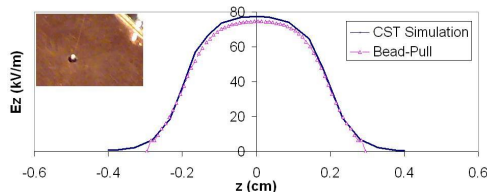
Figure 2: Bead-pull measurement of field strength compared with CST simulation results.
