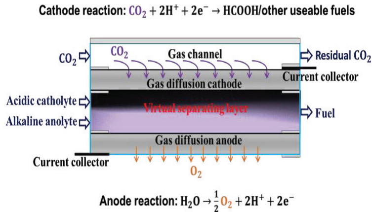
Fig. 1 Schematic diagram of a DEMR (N.B. the virtual separating layer is identified by fluorescein microscopy)
