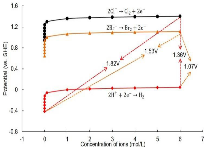
Fig. 3 Pourbaix diagram of \text{H}_2 , \text{Cl}_2 and \text{Br}_2 electrode reactions at room temperature
