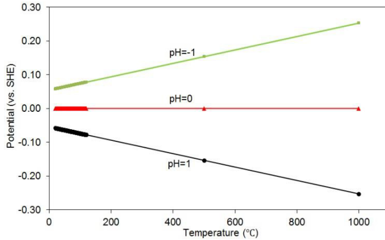
Fig. 2 Pourbaix diagram of the hydrogen electrode
