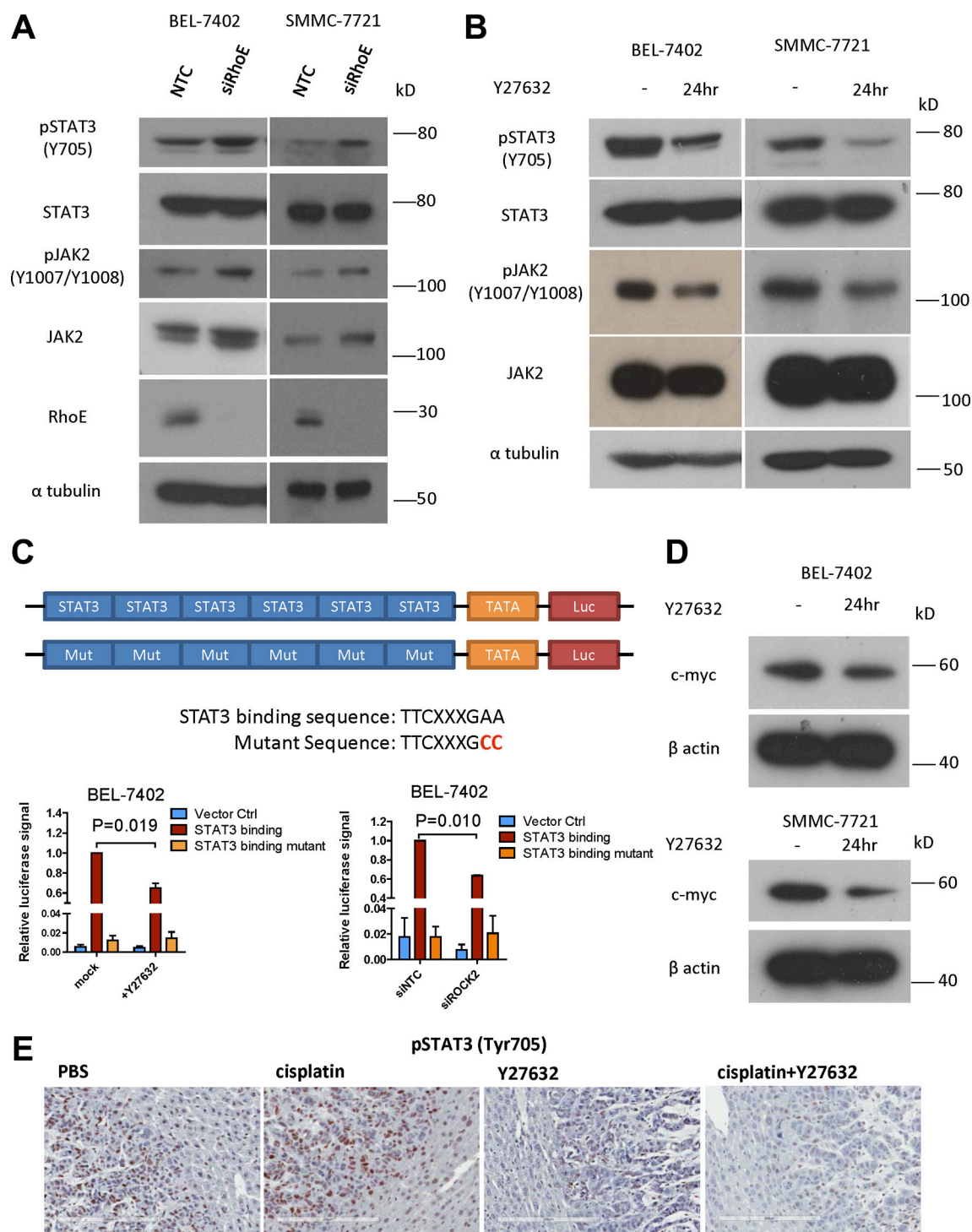
Figure 4: Inhibition of ROCK repressed the activity of JAK2 and STAT3. (A) Knockdown of RhoE by siRNA induced phosphorylation of both JAK2 and STAT3 in BEL-7402 and SMMC-7721 cells. (B) Treatment with Y27632 for 24 hours inhibited the phosphorylation of JAK2 and STAT3 in BEL-7402 and SMMC-7721 cells. (C) Schematic diagram showing the construct which expressed firefly luciferase under the control of STAT3-binding elements. Both Y27632 and ROCK2 knockdown by siRNA reduced the luciferase activity in BEL-7402 cells. SV40-driven expression of Renilla luciferase was used as normalization control. (D) Treatment with Y27632 for 24 hours decreased the protein level of c-myc, a transcriptional target of STAT3, in BEL-7402 and SMMC-7721 cells. (E) Representative IHC staining of p-STAT3 (Y705) in xenograft tumors harvested from subcutaneous tumor injection model (Figure 3B). Y27632 remarkably diminished the p-STAT3 (Y705) signals; the p-STAT3 stain was nearly totally abolished in the combined Y27632 and cisplatin treatment group. Original magnification, \times 20 ; scale bars: 200 \mu\text{m} . 10 \mu\text{M} Y27632 was used. In all panels, 3 experiments are represented. P -value was calculated using Student's t test.
