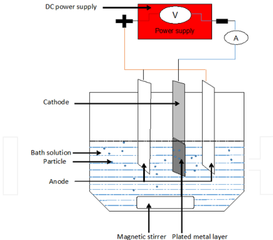
Figure 3. Typical Electrolytic Cell for Electrodeposition of Metals
