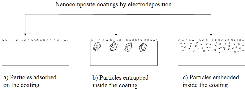
Figure 5. Schematic Representation of Different Codeposition Possibilities
