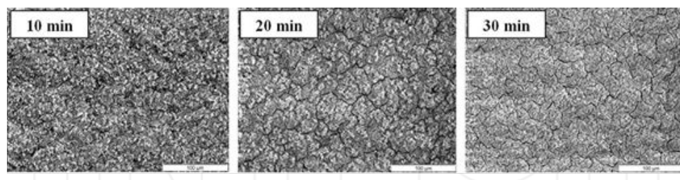
Figure 8. Surface Morphology of Electrodeposited Films with Increasing Time at Room Temperature in 0.1 mol/L Ce(NO 3 ) 3 ·6H 2 O for an Applied Density of –1 mA/cm 2 [32].
